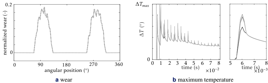
Figure 8. Convergence analysis of the wear and temperature profiles with the number of thermal abrasable coating elements n_{ab,th} . n_{ab,th} = 50 or R_s = 400 (—), n_{ab,th} = 100 or R_s = 200 (—), n_{ab,th} = 50 or R_s = 400 (—), n_{ab,th} = 800 or R_s = 25 (—)
