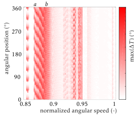
Figure 13. Temperature map at the trailing edge
