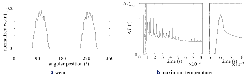
Figure 9. Convergence analysis of the wear and temperature profiles R_t . R_t = 1 (—), R_t = 5 (—), R_t = 10 (—), R_t = 15 (—), R_t = 20 (—), R_t = 25 (—), R_t = 50 (—), R_t = 100 (—), R_t = 150 (—), R_t = 200 (—), R_t = 300 (—)
