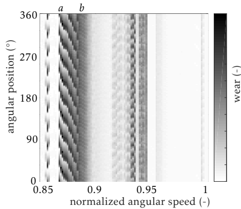
Figure 12. Wear map at the trailing edge
