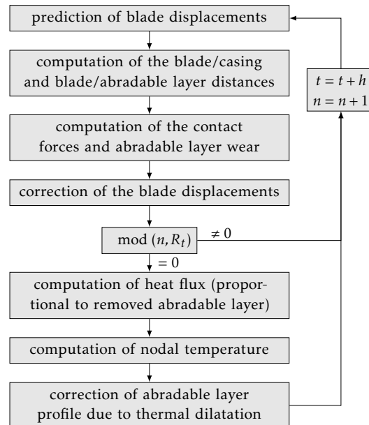
Figure 3. Flow chart of the time integration algorithm
