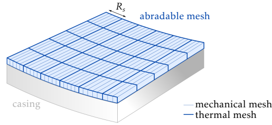
Figure 2. Spatial discretization of the abrasible coating mesh
