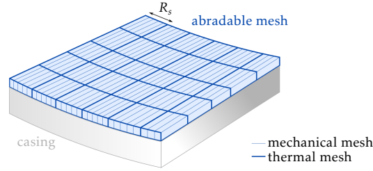
Figure 2. Spatial discretization of the abradable coating mesh
