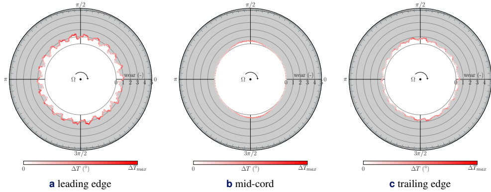
Figure 7. Wear and temperature profiles at 0.51 s
