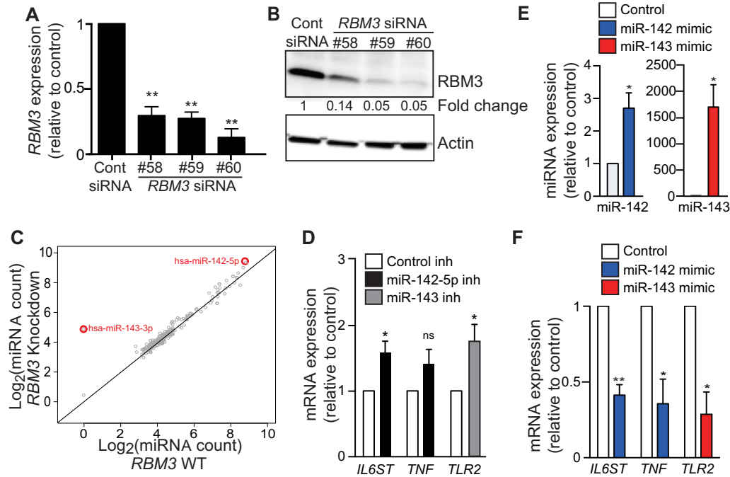
Figure 4. RBM3 siRNA knockdown increases the expression of thermomiRs. (A) Expression of RBM3 mRNA by RT-qPCR, and (B) RBM3 protein levels by Western blot in THP-1-derived macrophages nucleofected with negative control siRNA and each of the three siRNAs against RBM3 : #58, #59 and #60. (C) Average counts of individual miRNAs from the three RBM3 knockdown experiments as measured using NanoString nCounter. Two miRNAs miR-142 and miR-143 showed the greatest change in expression. (D) Expression of pyrogens in THP-1-derived macrophages: IL6ST , TNF and TLR2 following inhibition of miR-142-5p and miR-143 (relative to control inhibitor). (E) Expression of miR-142 and miR-143 in THP-1-derived macrophage at 24 h after nucleofection with respective miRNA mimics (relative to control). (F) Expression of IL6ST , TNF and TLR2 in THP-1-derived macrophage at 24 h following nucleofection of miR-142 and miR-143 mimic (relative to control). Data are from three independent experiments each in triplicate and show mean ± SEM. Two-tailed Student’s t -test was used to determine significance, denoted by * ( P < 0.05 ) and ** ( P < 0.001 ). inh, inhibitor; ns, not significant.
