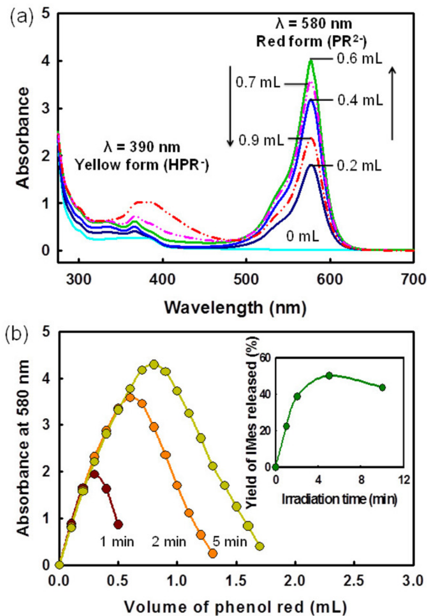
Figure 5: Quantification of IMes amount released. (a) Change of UV-Vis spectra of an acetonitrile solution of \text{IMesH}^+\text{BPh}_4^- ( 3.0 \times 10^{-4} M) and ITX ( 1 \times 10^{-4} M) irradiated for 2 min (LED, 365 nm, 65 \text{ mW cm}^{-2} ) upon gradual addition of PR ( 2 \times 10^{-4} M); (b) titration plot showing the absorbance at 580 nm for the same solution irradiated at 1, 2, or 5 min as a function of PR (titrant) volume. The insert gives the yield of photogenerated NHCs deduced from the spectrophotometric titration curve. This figure has been modified from a previous publication 9 . Please click here to view a larger version of this figure.
