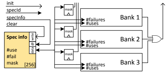
Fig. 2. Global view of the Partitioned Load Store Queue with three banks
