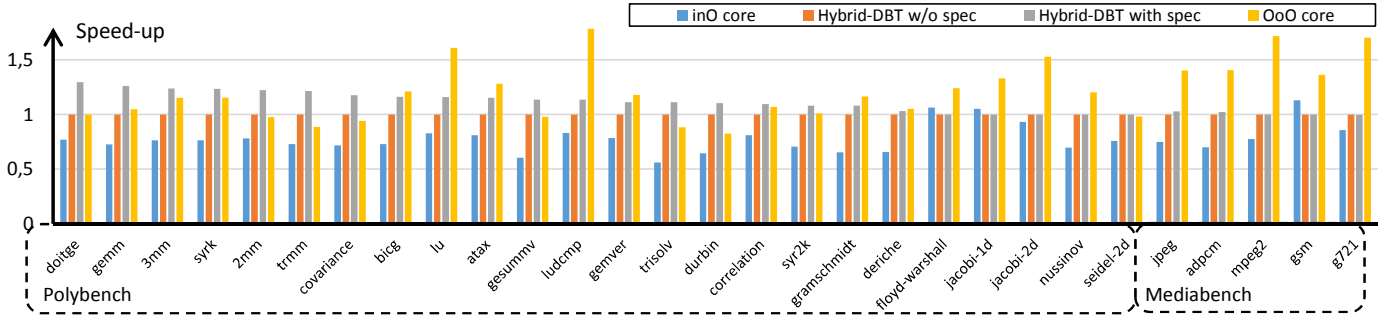
Fig. 4. Speed-up for the different applications, using the non-speculative Hybrid-DBT as a baseline (higher is better)
