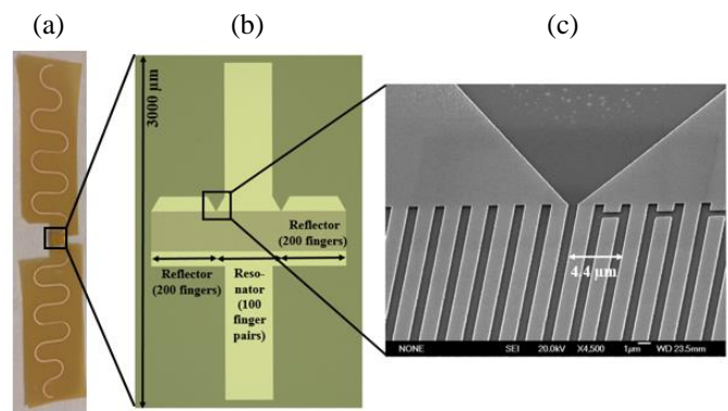
Fig. 2. Top view of finale structure, including the sensor and a flexible antenna (a), and the fabricated SAW device (b and c)
