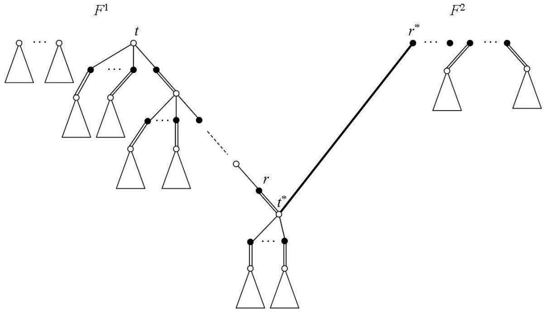
Figure 2: Case 1: augmenting path (t, \dots, t^*, r^*) .
