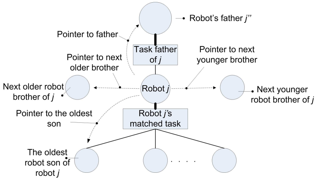
Figure 6: The pointers to the (robot) neighbors of a robot j .
