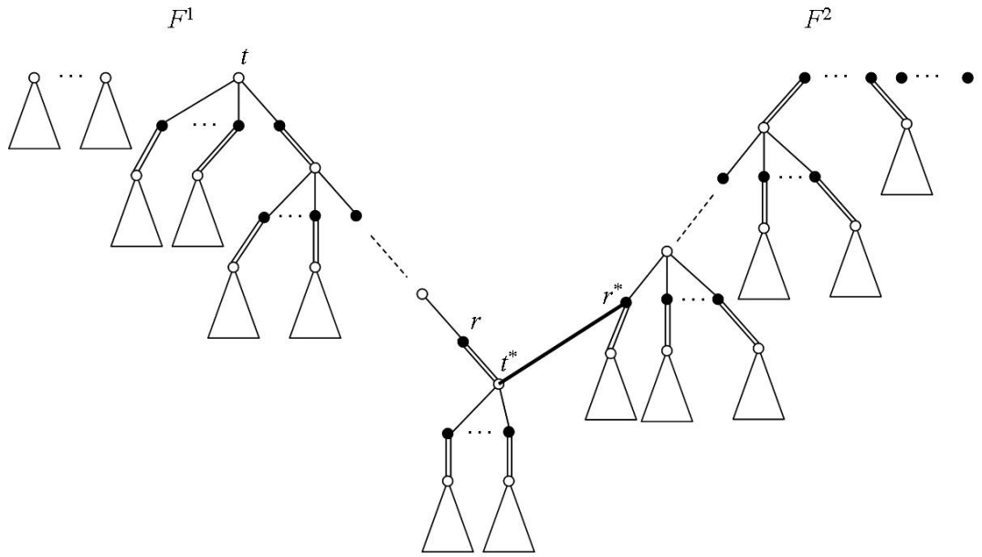
Figure 4: Case 2: no new augmenting path.
