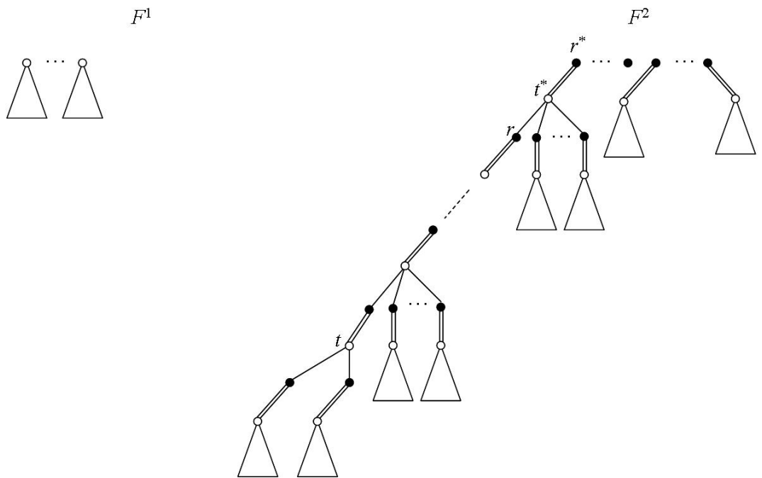
Figure 3: Case 1: forests' updating.
