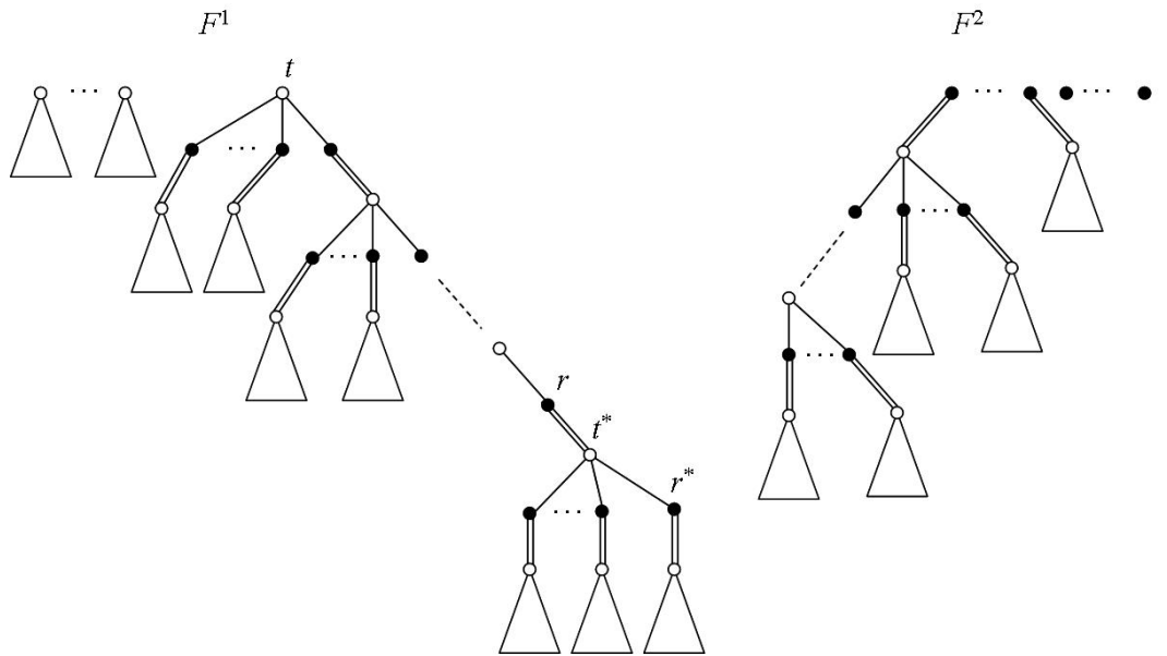
Figure 5: Case 2: forests' updating.
