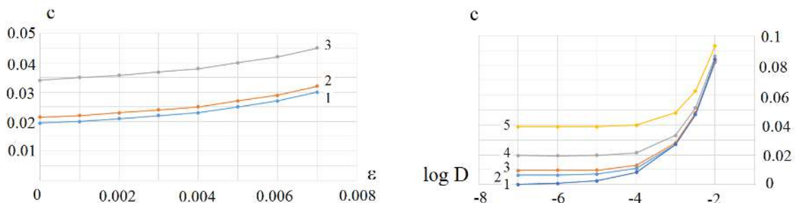
Figure 2: Dependence of the wave speed on \epsilon (left) and on D (right). The values of parameters are as follows: k = 0.1, r = 20, \phi_0 = 10, b = 0.05, u_0 = 0.1 , 1. D = 10^{-6} , 2. D = 10^{-4} , 3. D = 10^{-3} (left); k = 0.1, b = 0.05, u_0 = 0.1, \epsilon = 10^{-5}, r = 2\phi_0 ; 1. analytical formula (4.6), 2. \phi_0 = 30 , 3. \phi_0 = 20 , 4. \phi_0 = 10 , 5. \phi_0 = 5 (right).
