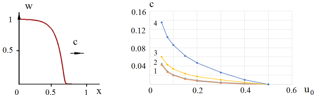
Figure 1: Numerical simulation of wave propagation. A snapshot of solution (left) and the wave speed dependence on the parameter u_0 (right) found numerically and by the analytical formula (4.5). The curves are obtained for different values of the diffusion coefficient: 1. D = 10^{-6} , 2. D = 10^{-4} , 3. D = 10^{-3} , 4. D = 10^{-2} . The values of other parameters are as follows: k = 0.1, b = 0.1, r = 20, \phi_0 = 10 . The analytical curve coincides with curve 1.
