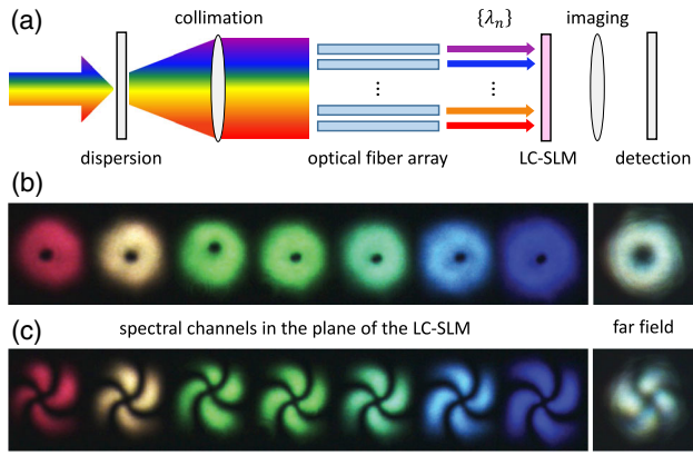
FIG. 3. (a) Sketch of the experimental setup for ultrabroadband scalar and vectorial vortex beam shaping. The optical fiber array consists of 12 multimode step-index fibers with numerical aperture 0.2 and core radius 50 \mu\text{m} . The detection system is either a camera or a fiber spectrometer. Scalar vortex (b) and vectorial (c) beam shaping when incident light is, respectively, circularly and linearly polarized. In both cases, the observation is made by placing an output polarizer that selects the polarization state orthogonal to the incident one. The image on the left corresponds to the seven spectral channels \lambda_n = 485, 511, 533, 555, 575, 595, and 617 \text{ nm} with \sim 10 \text{ nm} full width at half maximum in the plane of the LC-SLM and the image on the right refers to the far field of the polychromatic structured light field.
