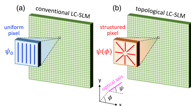
FIG. 1. (a) Illustration of a usual optical device made of a two-dimensional matrix of electrically controlled liquid crystal pixels having a uniform molecular orientation, \psi = \psi_0 . (b) Topological counterpart where every pixel acts as an electrically controlled microscopic q plate ( q = +1 for the enlarged pixel).
