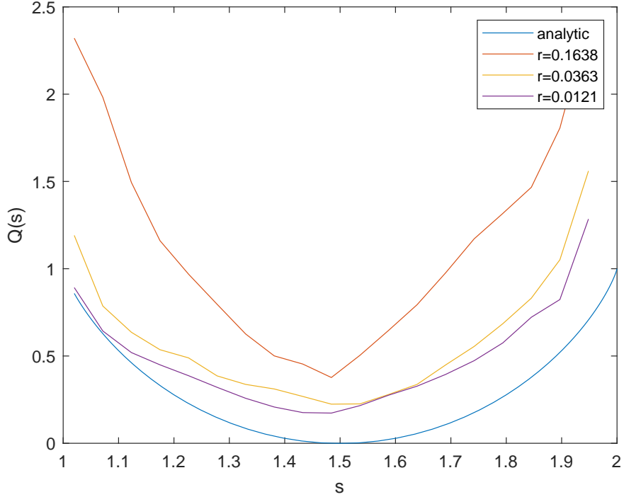
Figure 5: Rate function Q(s) for the motion on a Sierpinski gasket, computed from 1,000 sampling points, each of which required a trajectory consisting of 10^6 iterates.
