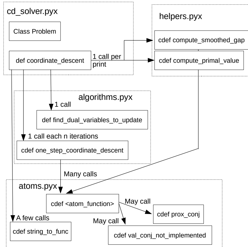
Figure 1: Code structure
