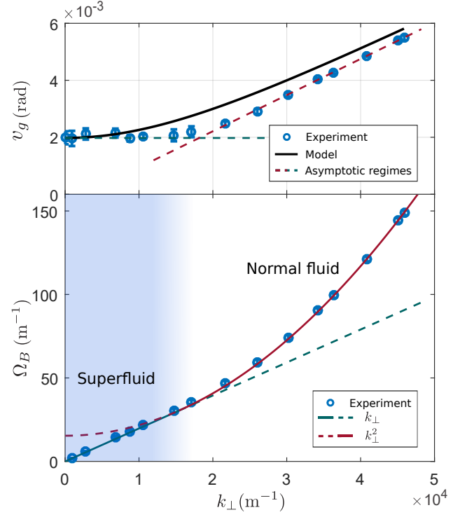
Figure 3. a) Group velocity as a function of k_\perp . + The circles represent the experimental data obtained for P = 175 mW. The theoretical model is plotted in black (no free parameter – see text for details). The dashed lines figure the asymptotic behaviors: constant group velocity at small k_\perp and linear increase at large k_\perp . b) Dispersion relation obtained after integration of the group velocity. Linear (blue) and parabolic (red) dispersion curves are plotted as a reference.
