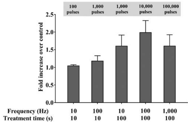
Fig. 6. Analysis of RONS production 30 min after plasma treatment using DHR 123 fluorescent probe. Results are expressed as fold increase over untreated control ( n = 3 ).
