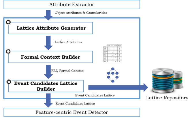
Fig. 5: The Event Candidates Lattice Builder module
