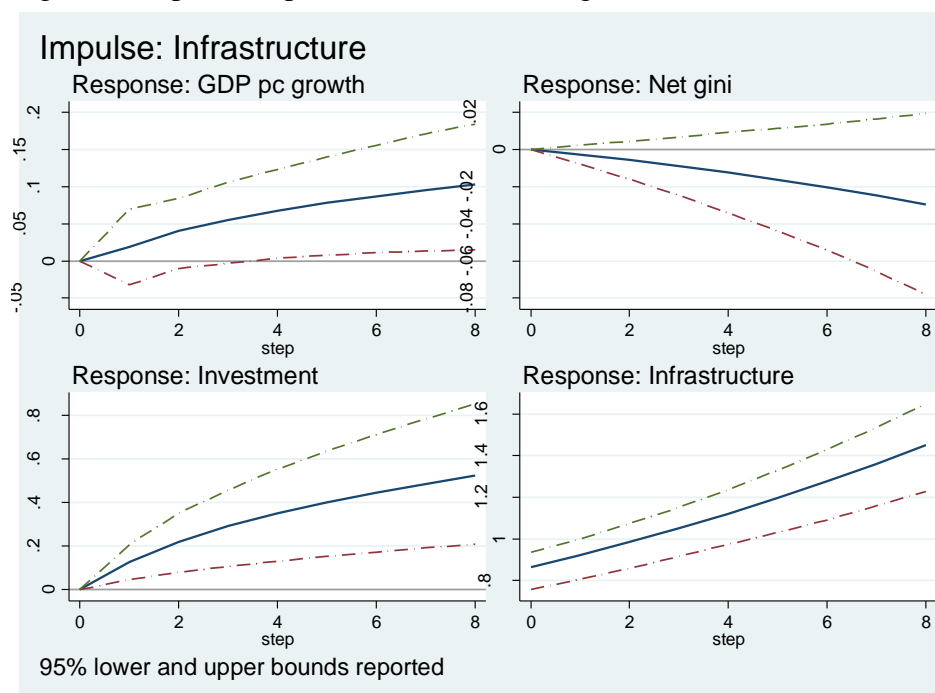
Figure 8: Impulse response functions – change in infrastructure
