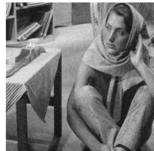
(i) Our result, k=0.3 , h=0.1 , \mu=5 , \lambda=1 , 20 iterations
