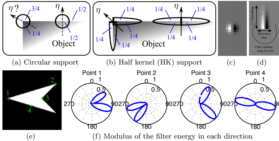
Fig. 2. Representation of filter supports concerning edges and corners. (c) Derivative Gaussian kernel. (d) 2D half kernel. (e) Selection of points before applying the HK_\theta .
