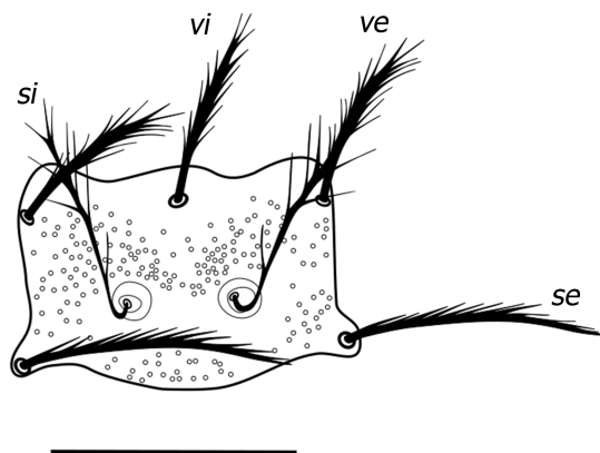
Figure 2 Morphological details of Eutrombicula daemoni n. sp. prodorsal sclerite. Symbols: ve = anterolateral setae; se = posterolateral setae; vi = anteromedial seta; si = trichobothria. Scale: 50 \mu\text{m} .
