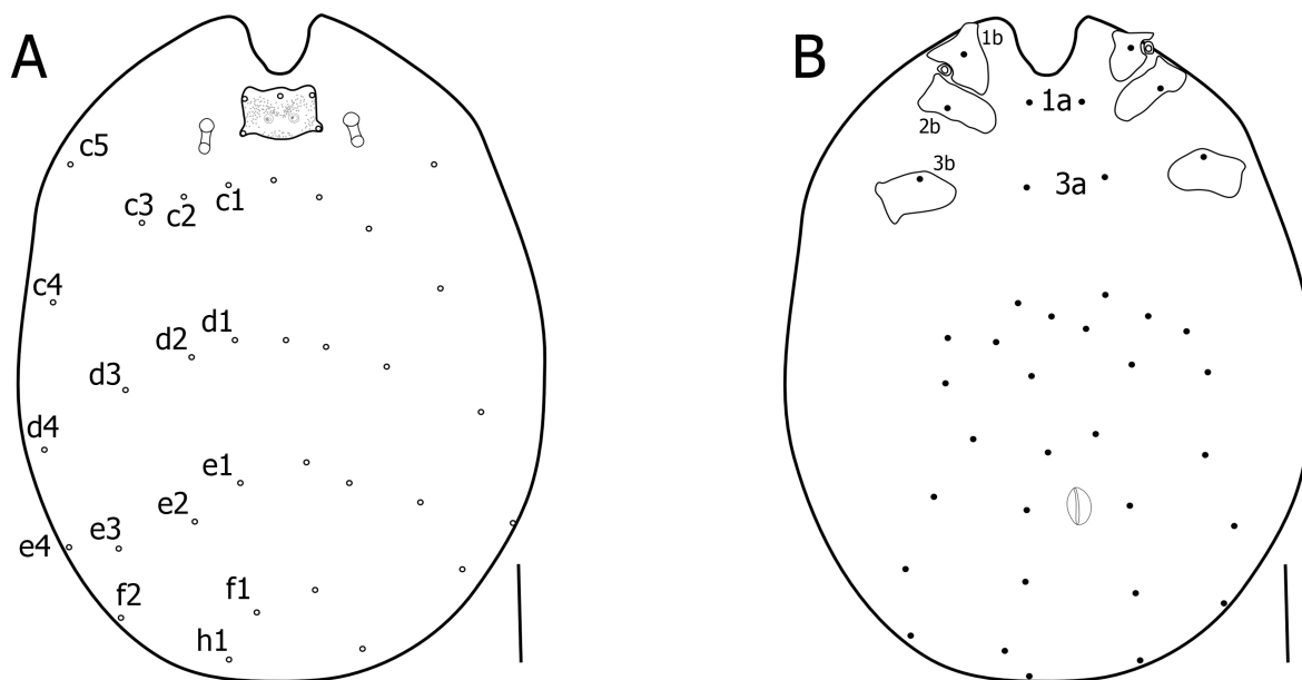
Figure 3 Morphological details of Eutrombicula daemoni n. sp. A. dorsal view of idiosoma; B. ventral view of idiosoma. Black spots = ventral setae of the idiosoma; white spots = dorsal setae of the idiosoma. Symbols: c1-c5 = setae of the C row; d1-d4 = setae of the D row; e1-e4 = setae of the E row; f1-f2 = setae of the F row; h1 = setae of the H row; 1a = anterior sternal setae; 3a = posterior sternal setae; 1b = seta of the coxal field of the leg I; 2b = seta of the coxal field of the leg II; 3b = seta of the coxal field of the leg III; Scales: A and B 100 \mu\text{m} .
