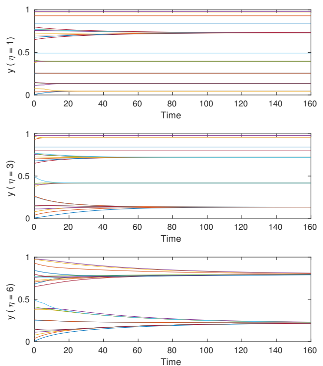
Fig. 2. Simulated evolutions of the state y with n = 25 and \varepsilon = 0.001 , starting from a randomly generated initial condition with 3 connected components. The parameters \eta are chosen in \{1, 3, 6\} and the resulting dynamics respectively lead to 11, 7 and 2 connected components in the final graph.
