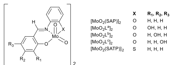
Scheme 2. Pre-catalysts used in this study
