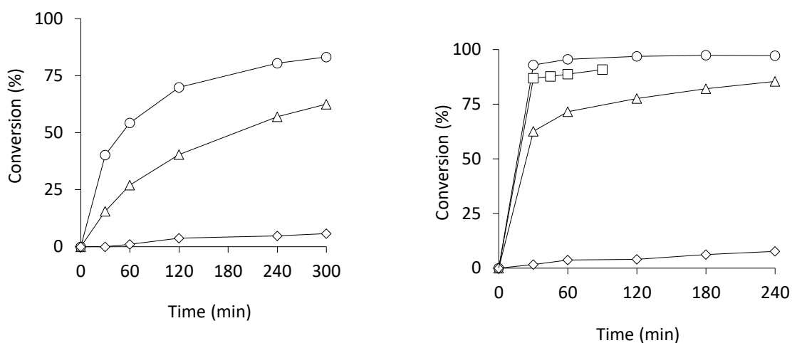
Figure 6. Influence of the catalyst loading on the [\text{MoO}_2(\text{SATP})]_2 -catalyzed limonene oxidation at 50°C (left) and 80°C (right): [\text{Mo}]/\text{limonene}/\text{TBHP} = x/100/200 , x = 0 (◇), 0.1 (△), 0.25 (□), 0.5 (○).
