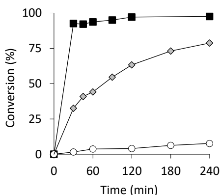
Figure 1. Kinetic profiles for limonene oxidation: without catalyst (O), with [MoO 2 (SAP)] 2 (◇), with [MoO 2 (SATP)] 2 (■). [Mo]/limonene/TBHP = 0.5/100/200, T = 80°C.
