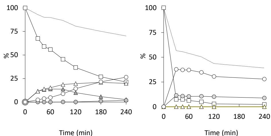
Figure 2. Kinetic profile for the limonene oxidation catalyzed by [\text{MoO}_2(\text{SAP})]_2 (left), [\text{MoO}_2(\text{SATP})]_2 (right): [\text{Mo}]/\text{limonene}/\text{TBHP} = 0.5/100/200 , T = 80^\circ\text{C} . Mass balance (...), limonene ( \square ), cis -LimO ( \blacktriangle ), trans -LimO ( \triangle ), eq -LimD ( \bullet ), ax -LimD ( \circ ).
