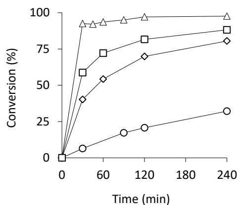
Figure 5. Influence of temperature on the [\text{MoO}_2(\text{SATP})]_2 -catalyzed limonene oxidation: 30°C (O), 50°C (◇), 60°C (□), 80°C (△). Conditions: [\text{Mo}]/\text{limonene}/\text{TBHP} = 0.5/100/200 .
