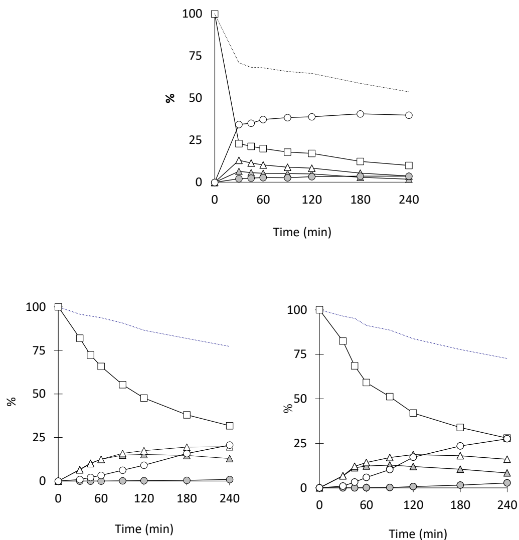
Figure 4. Kinetic profile for the limonene oxidation catalyzed by [\text{MoO}_2\text{L}^{\text{a}}]_2 (up), [\text{MoO}_2\text{L}^{\text{b}}]_2 (down left), [\text{MoO}_2\text{L}^{\text{c}}]_2 (down right),: [\text{Mo}]/\text{limonene}/\text{TBHP} = 0.5/100/200 , T = 80^\circ\text{C} . Mass balance (...), limonene ( \square ), cis -LimO ( \blacktriangle ), trans -LimO ( \triangle ), eq -LimD ( \bullet ), ax -LimD ( \circ ).
