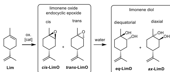
Scheme 1. Oxidation of limonene and potential LimO and LimD products.
