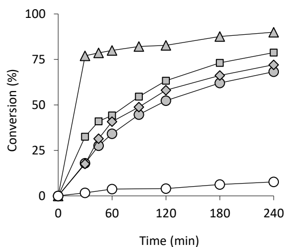
Figure 3. Kinetic profile for limonene oxidation: without catalyst (–), with [\text{MoO}_2(\text{SAP})]_2 (■), with [\text{MoO}_2\text{L}^a]_2 (▲), with [\text{MoO}_2\text{L}^b]_2 (●), with [\text{MoO}_2\text{L}^c]_2 (◆). [\text{Mo}]/\text{limonene}/\text{TBHP} = 0.5/100/200 , reaction time = 4 h, T = 80^\circ\text{C} .
