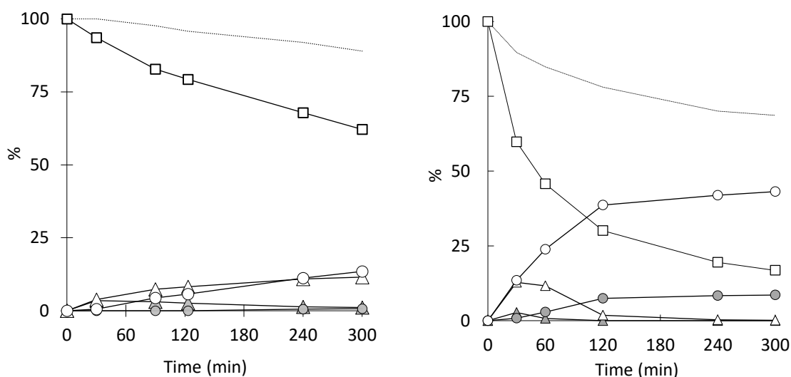
Figure 7. Kinetic profile for the limonene oxidation catalyzed by [\text{MoO}_2(\text{SATP})]_2 at 30°C (left) and 50°C (right): [\text{Mo}]/\text{limonene}/\text{TBHP} = 0.5/100/200 . Mass balance (...), limonene (□), cis -LimO (▲), trans -LimO (△), eq -LimD (●), ax -LimD (○).
