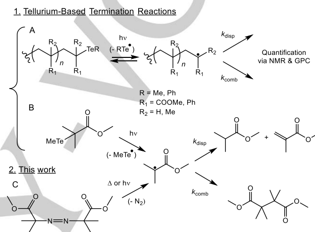
Scheme 1. 1 (top): work using organotellurium initiators to generate carbon-based radicals from (A) TERP macroinitiators and (B) the unimer model of the pMMA-TeMe dormant species. [6] 2 (bottom): activation of the diazo compound V-601 to generate methacrylate radicals in the absence of tellurium compounds.
