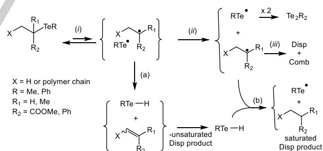
Scheme 2. Proposed mechanism for C-based radical disproportionation catalyzed by RTe • . (i) Radical pair generation; (ii) solvent cage escape; (iii) bimolecular radical termination
