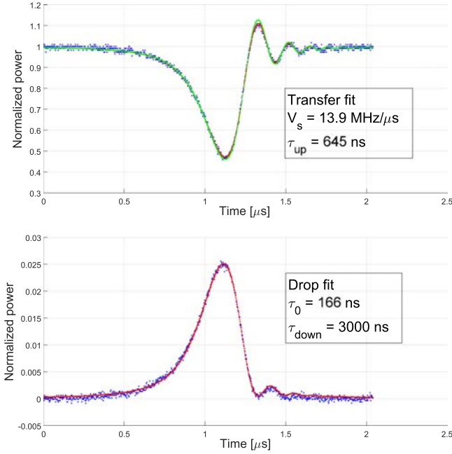
Figure 6. Typical results of the fitting procedure described in the main text. The red curves are the profiles obtained after the minimisation of \text{RSD}_{\text{tra}} and \text{RSD}_{\text{drp}} , while the green profile is the consistency plot ( s_{\text{tra}}^{\text{chk}} ).
