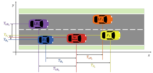
Figure 4: Diagram of the perception of our vehicles.
