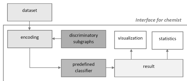
Figure 4: Schema of PREPEP’s workflow.
