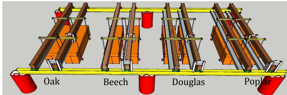
Fig 1: Creep device of service class 1
