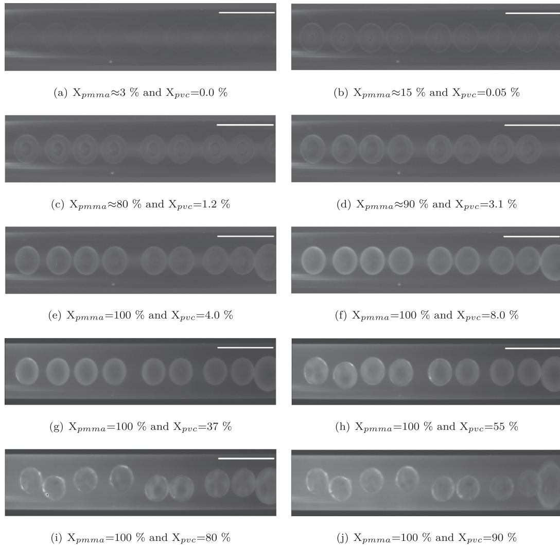
Fig. 12. Evolution of the droplets/particles during the MMA/VCM copolymerization. Experiment E4. Bar length = 530 \mu\text{m} .
