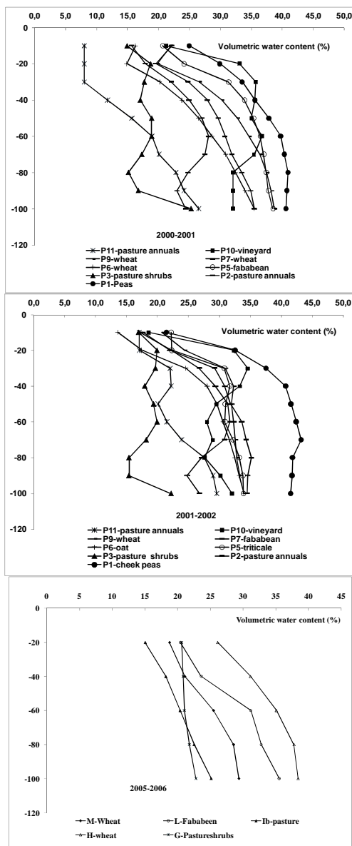
Figure 5. Variations of mean soil moisture profile in different seasons and land uses.
