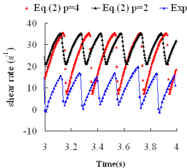
Fig(12) Comparison of two divergences of the viscosity (Eq.(2)) witheither p=2 (black triangles) or p=4 (red triangles) The blue triangles are tfrom experiment.
