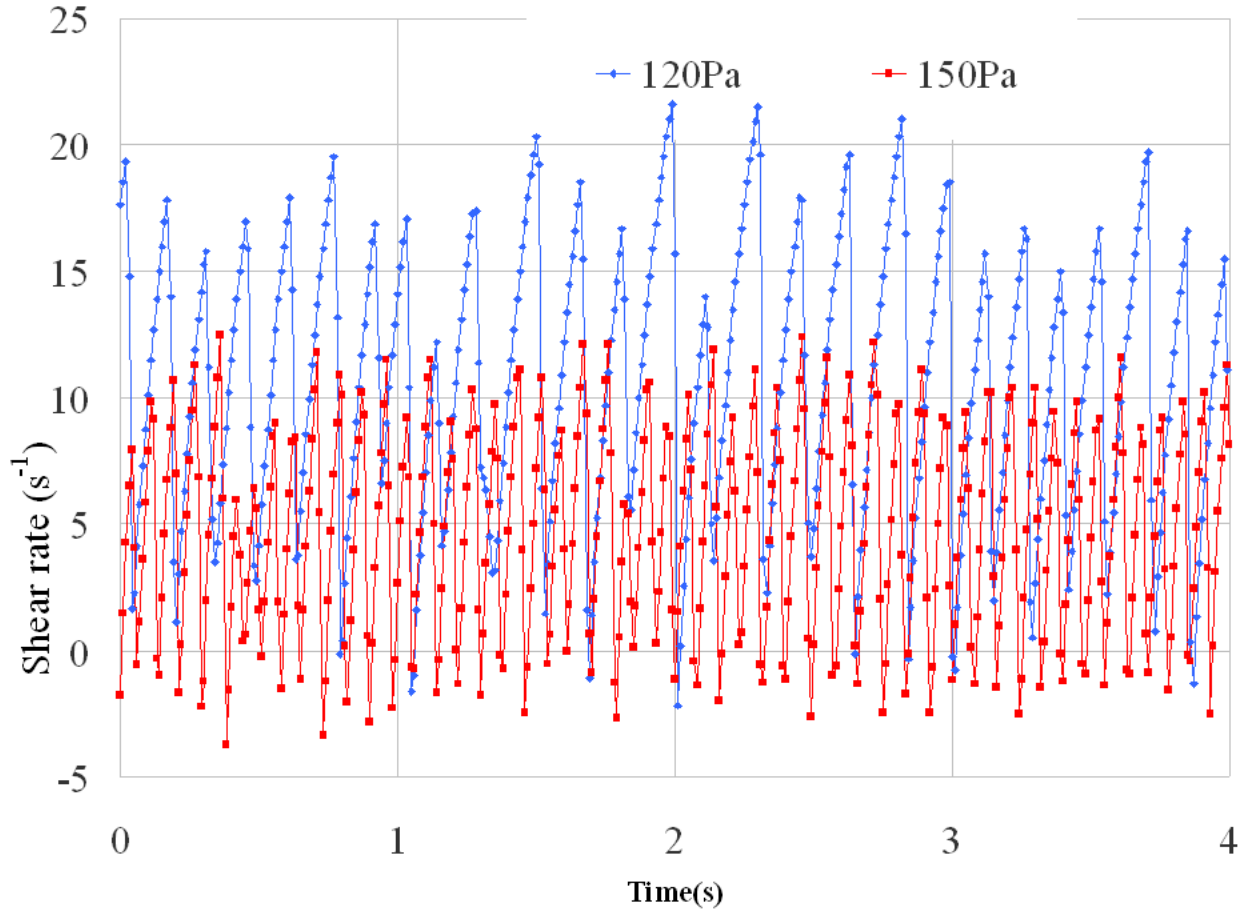
Fig.9 Shear rate versus time for a constant applied stress of 120 Pa and then 150Pa. Carboxy iron suspension at \Phi=0.62 with 0.2% weight of PPP44
