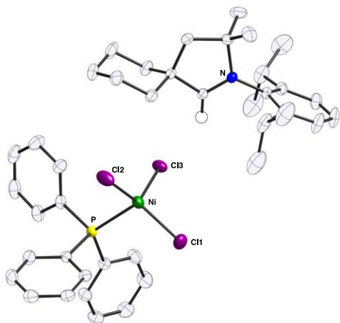
Figure 2. Structures of the cation and anion of 2a . Only the pyrrolidinylium H is shown (as a white isotropic sphere). Ellip-
