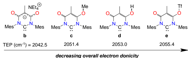
Figure 1. Electron-donicity of Mes- malo NHC Me -Mes ( b ), and of its electrophile-trapped derivatives. TEP values calculated from \nu(\text{CO})^{\text{av}} values measured for [RhCl(CO) 2 (NHC)] complexes. 13d
