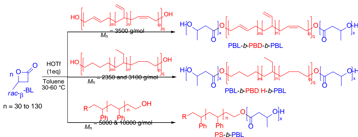
Scheme 1. Preparation of the PBL- b -PBD- b -PBL and PBL- b -PBD H- b -PBL triblock and PS- b -PBL diblock copolymers
