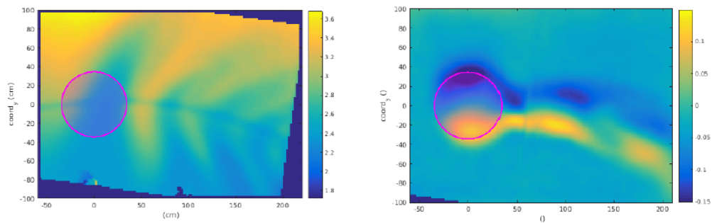
Figure: two horizontal cuts of the wake behind a spherical cap (whose basis is indicated by the circle) in the absence of background rotation: the waves measured at height z=60 cm from the tank bottom (left) and the eddies measured in the lower part at z=10 cm (right). The stream-wise velocity is mapped in the left side view (color scale in cm/s) while the vorticity is mapped in the right side view (color scale in s -1 ). Both fields are averaged during 1 minute.
