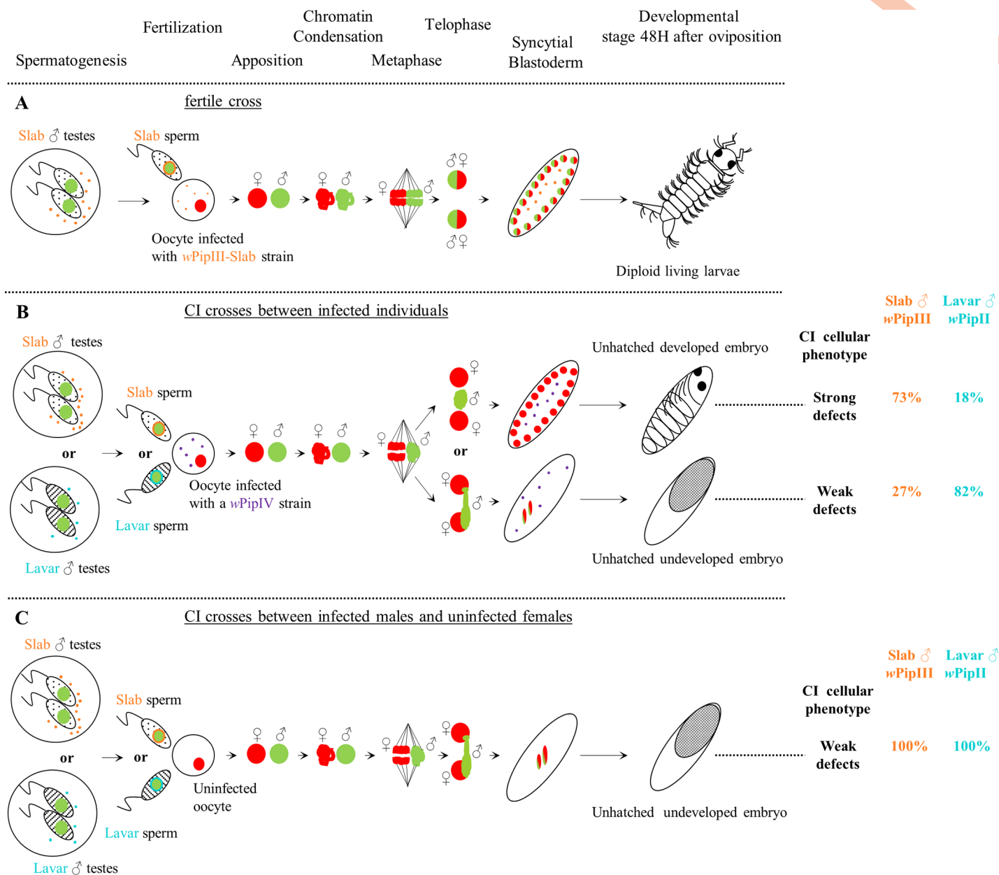
Fig 6. Cellular bases of different developmental fates in C. pipiens : From spermatogenesis to late developmental stages. Paternal and maternal DNA are represented in green and red respectively and Wolbachia cells are represented by the small dots (blue for wPipII; orange for wPipIII and purple for wPipIV). The two MAL lines Slab and Lavar have been chosen to illustrate the variability in CI defects intensity (i.e. frequency of strong and weak cellular CI). During spermatogenesis, the Wolbachia in male testes produce a toxin ( mod factor). After fertilization, if females and males are infected with the same Wolbachia (Panel A), they can prevent the toxicity ( resc function) and allow normal embryogenesis and the production of living diploid larvae. However, if the Wolbachia in the females are incompatible with the Wolbachia in the males (Panel B) or absent (Panel C) then the toxicity would not be prevented and paternal chromatin condensation delay and segregation defects occur. Two outcomes of the first zygotic division are possible regarding the degree of paternal chromatin exclusion. If the paternal chromatin is partially excluded, chromatid bridges would be formed resulting in aneuploid nuclei which might go through few mitotic divisions but will arrest the embryogenesis at early stages producing embryos with no visible development. If the paternal chromatin is fully excluded from the first zygotic division, maternal chromatin can segregate and produce two haploid nuclei which will divide further to produce non-viable haploid embryos exhibiting advanced development stages with eyes and segmentation clearly visible. The proportion of unhatched haploid embryos is influenced by different wPip with distinct mod profiles in the MAL lines involved in the crosses. However when the egg is not infected by Wolbachia (Panel C), all embryos exhibited an absence of further development after the first zygotic divisions whatever the mod induced by the wPip hosted by the MAL lines.
