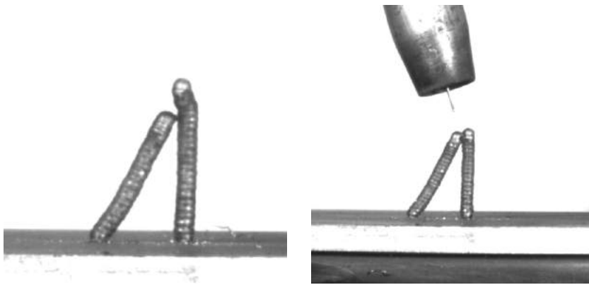
Figure 9: Left: Example of an aggregation of deposition on the right skeleton freeform shape; Right: Example of reorientation of the welding torch to avoid the obstruction problem.
