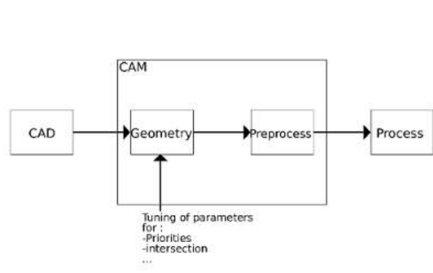
Figure 2: Numerical chain for WAAM
