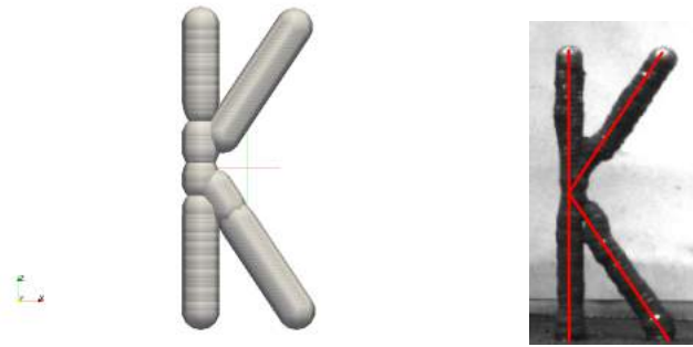
Figure 13: Left: Targeted virtual K shape with ratio management ; Right: K shape freeform manufactured sample. In red full line is represented the virtual CAD definition.
