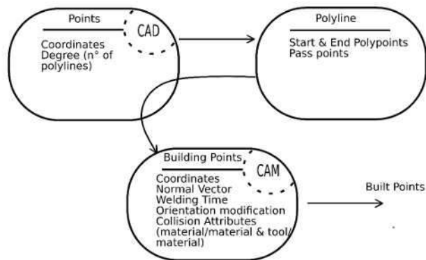
Figure 4: Connection between points and polylines for the manufacturing of skeleton freeform shapes.
