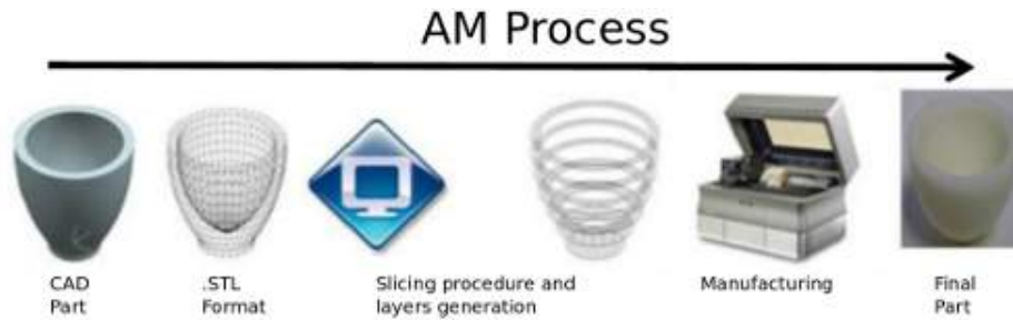
Figure 1: Computer Aided Design (CAD) ; Generation of a STL file ; Slicing of the file into layers ; Generation of the trajectories ; Manufacturing of the part [4].
