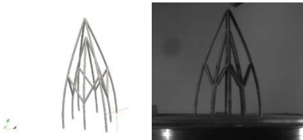
Figure 14: Left: Targeted virtual structure including convergent and divergent intersections ; Right: 3D manufactured structure sample.
