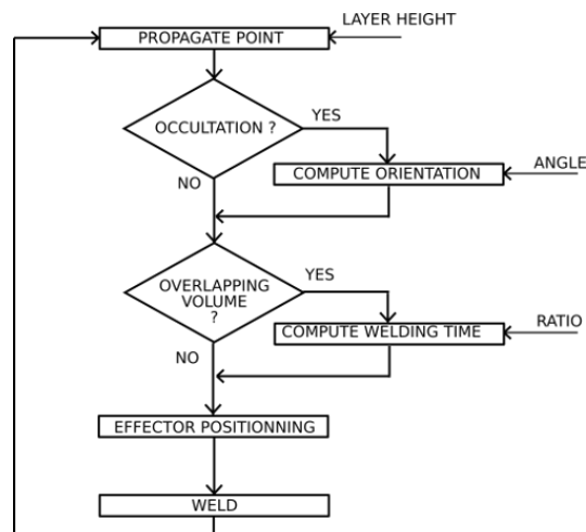
Figure 11: Functioning of our CAM software for intersection areas.
