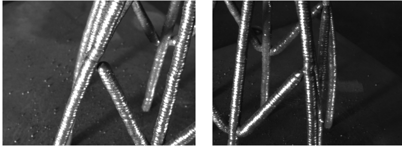
Figure 15: Left: Intersection with a bad deposition (lack of material); Right: Intersection with a better filling.
