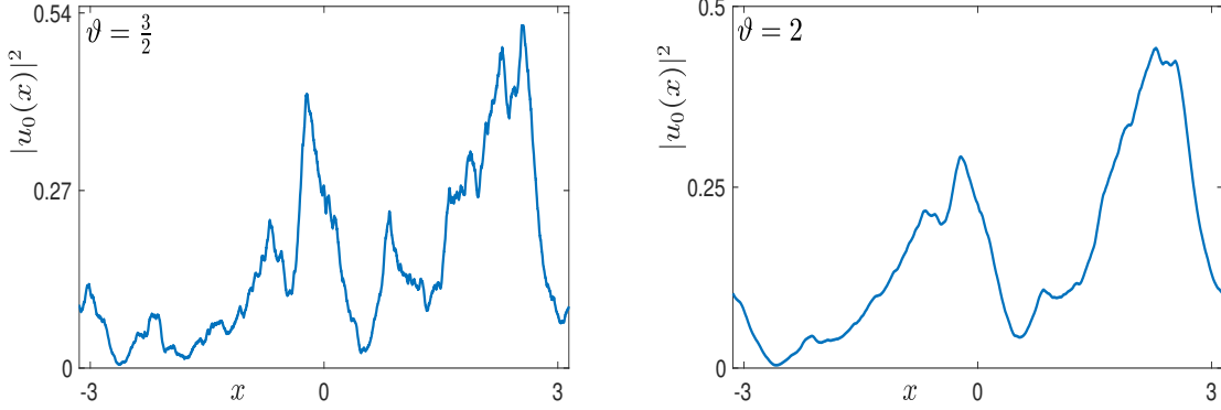
FIGURE 4.1. Initial data (4.2) for \vartheta = \frac{3}{2} (left) and \vartheta = 2 (right).
