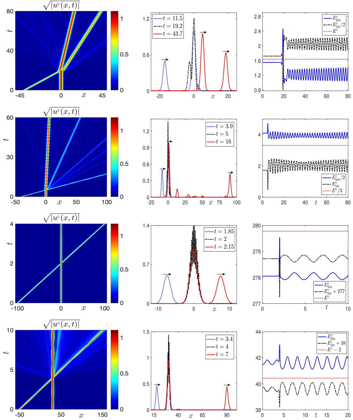
FIGURE 4.6. Plots of \sqrt{|u^\epsilon(x,t)|} (first column), |u^\epsilon(x,t)| at different time (second column) and evolution of the energies (third column) for different parameters in Example 3 : Case v–Case viii (from top to bottom).
