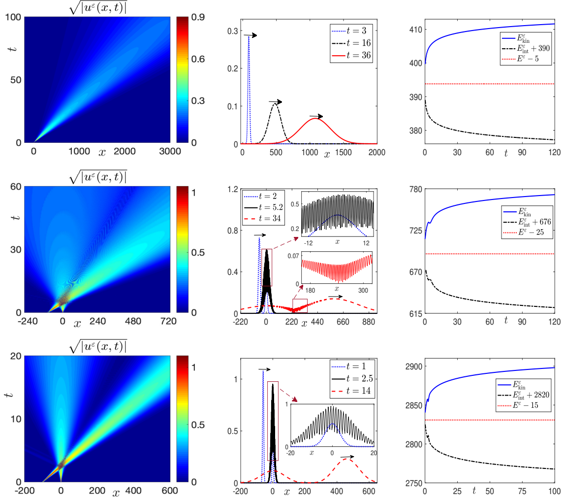
FIGURE 4.7. Plots of \sqrt{|u^\epsilon(x,t)|} (first column), |u^\epsilon(x,t)| at different time (second column) and evolution of the energies (third column) for different parameters in Example 4 : Cases ix–xi (from top to bottom).
