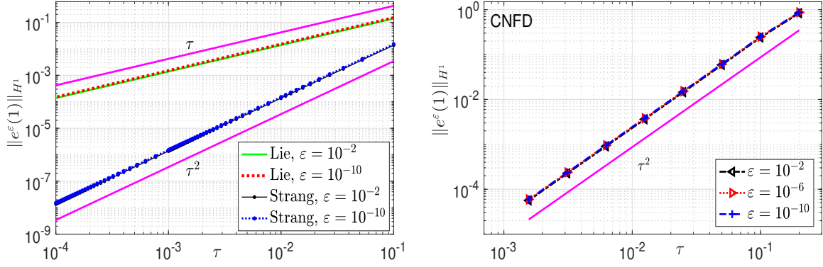
FIGURE 4.2. Errors \|e^\varepsilon(1)\|_{H^1} of LTSP & STSP (left) and CNFD (right) for Case I.
