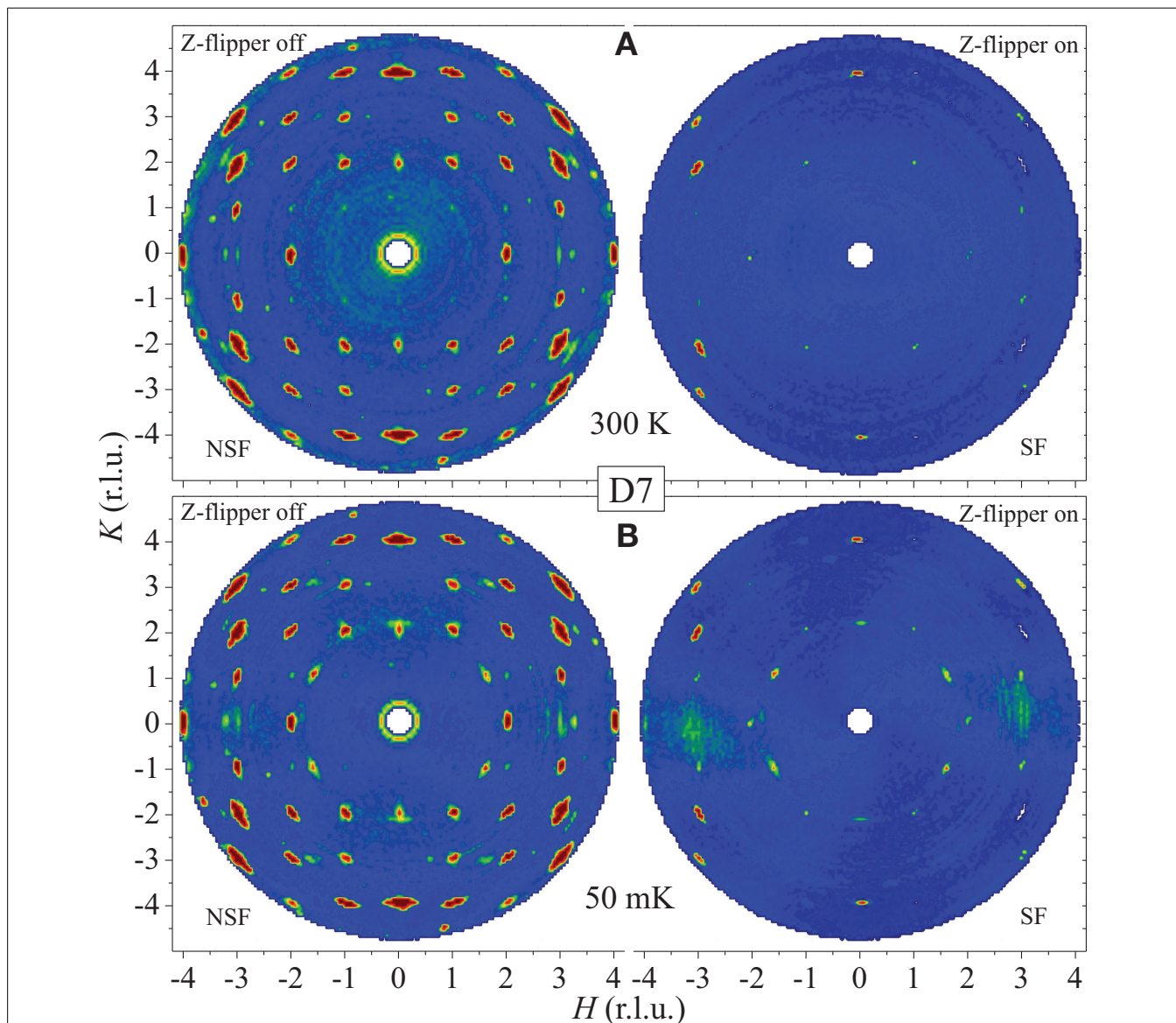
FIGURE 1 | Polarization analysis data measured using D7 (ILL). (A) At 300 K. (B) At 50 mK. The NSF (i.e., Z-flipper off, left panel) and SF (i.e., Z-flipper on, right panel) channels are shown with the same color code for intensity. The non-perfect polarization involuntarily leads to the presence of some nuclear Bragg peaks, e.g., (0, \pm 4, 0) , in the SF channel at both
