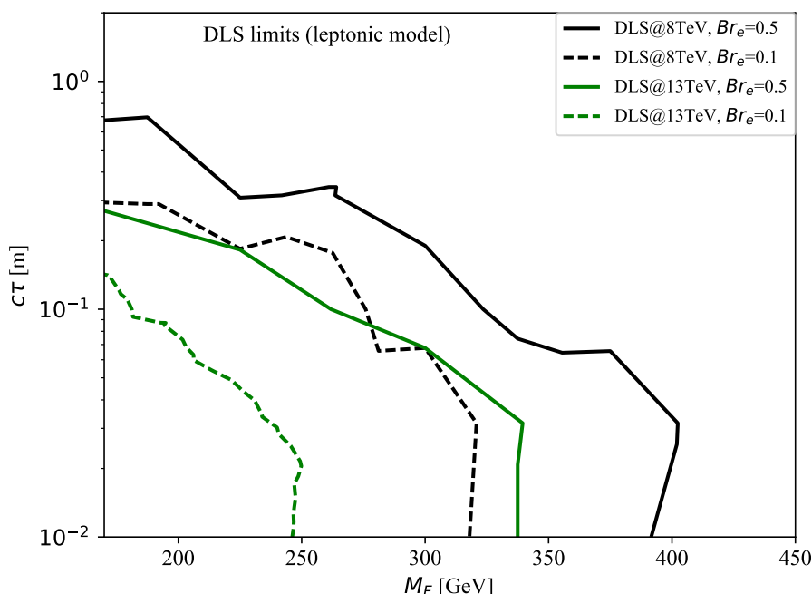
Figure 5. 95 % C.L. exclusions in the c\tau vs m_F plane due to the 8 TeV ( 19.7\text{ fb}^{-1} , black) and 13 TeV ( 2.6\text{ fb}^{-1} , green) CMS Displaced Lepton searches. The solid curve indicates the case where Br(F \rightarrow es) \equiv Br_e = 0.5 and Br(F \rightarrow \mu s) \equiv Br_\mu = 0.5 , while the dashed line denotes the case where Br_e = 0.1 and Br_\mu = 0.9 .
