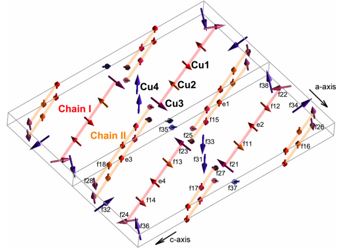
FIG. 6. Schematic representation of the AF structure of \text{La}_8\text{Cu}_7\text{O}_{19} . For clarity, only the Cu magnetic moments are shown. Two crystallographic units 2(a \times b \times c) are shown. The color type indicates the paired moments. Red-type colors denote moments constituting rungs, blue-type colors indicate moments situated in tetrahedral sites providing a connection between rungs. Two types of rungs with moments perpendicular to the b axis and along the b axis are shown by orange and red color and are denoted as Chain I and Chain II, respectively. All magnetic moments are labeled in agreement with Table II.
