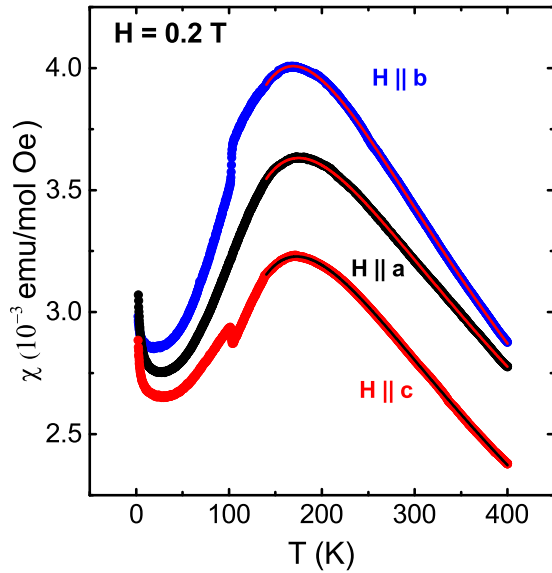
FIG. 4. Temperature dependence of the magnetic susceptibility \chi = M/H of \text{La}_8\text{Cu}_7\text{O}_{19} measured with field of 0.2 T applied along all three principal directions a , b , and c . Full lines through the points above 140 K are the best fits to the model described in the main text.
