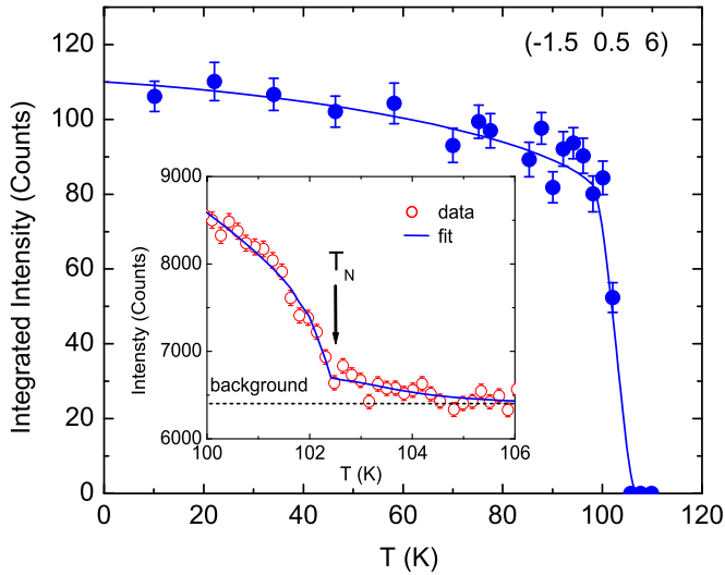
FIG. 5. Temperature dependence of the integrated intensity of the representative magnetic reflection (-\frac{3}{2}, \frac{1}{2}, 6) measured on the large \text{La}_8\text{Cu}_7\text{O}_{19} sample in zero field with increasing temperature. In the inset we show the temperature dependence of the peak intensity of the same reflection measured in a small temperature range around the magnetic phase transition. The best fit to the formula describing the decrease of the staggered magnetization in an antiferromagnet that includes a critical scattering [19] is shown by the full blue line.
