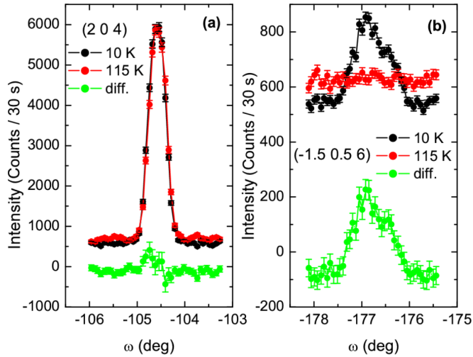
FIG. 2. Typical rocking curves of the nuclear Bragg reflection (2 0 4) at 10 K and 115 K, together with the difference between them (a) and of the magnetic Bragg reflection (-1.5 \ 0.5 \ 6) measured on the large sample for identical conditions (b). All measurements were scaled to the same monitor.
