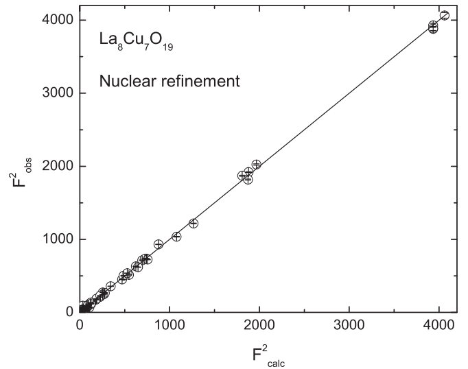
FIG. 3. Plot of the observed versus calculated squared nuclear structure factors collected on the large \text{La}_8\text{Cu}_7\text{O}_{19} single crystal after correction for the extinction and Lorentz factor, and refinement using the model shown in Fig. 6.
