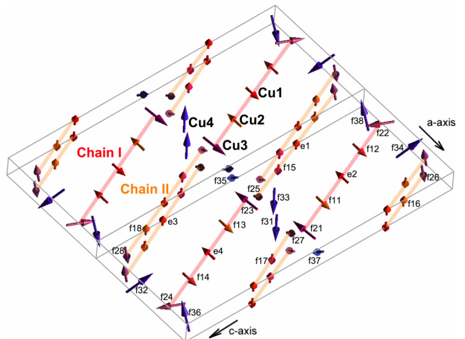
FIG. 6. Schematic representation of the AF structure of \text{La}_8\text{Cu}_7\text{O}_{19} . For clarity, only the Cu magnetic moments are shown. Two crystallographic units 2(a \times b \times c) are shown. The color type indicates the paired moments. Red-type colors denote moments constituting rungs, blue-type colors indicate moments situated in tetrahedral sites providing a connection between rungs. Two types of rungs with moments perpendicular to the b axis and along the b axis are shown by orange and red color and are denoted as Chain I and Chain II, respectively. All magnetic moments are labeled in agreement with Table II.
