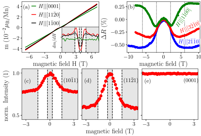
FIG. 7. Magnetic field sweeps performed using different methods. (a) Magnetic moment per Mn atom of MnTe on SrF 2 determined by SQUID for magnetic fields applied in various directions. The diamagnetic contribution of the substrate was subtracted. An inset shows the derivative of the magnetic moment by the magnetic field. For the in-plane measurements distinct regions are detected which are distinguished by the slope of m(T) . (b) Change of the longitudinal resistance in MnTe on InP(111) measured in Corbino disk geometry vs magnetic field applied along the [2\bar{1}\bar{1}0] , [3\bar{2}\bar{1}0] , and [1\bar{1}00] directions. (c)–(e) Normalized neutron diffraction intensity of the (10\bar{1}\bar{1}) , (11\bar{2}\bar{1}) , and (0001) Bragg peak of MnTe grown on SrF 2 during a magnetic field sweep with field along the [1\bar{1}00] direction.
