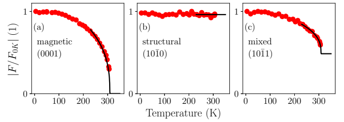
FIG. 4. Neutron diffraction structure factors measured vs temperature for the (a) magnetic (0001), (b) structural (10 \bar{1} 0), and (c) mixed structural and magnetic Bragg peak (10 \bar{1} 1). Black lines show the behavior close to the Néel temperature described by the equation A_{\text{mag}}(T_N - T)^c + A_{\text{struct}} , where A_i denotes the amplitude of magnetic and structural contribution and T the measurement temperature. The Néel temperature T_N = 309 K and the critical exponent c = 0.37 corresponds to the Heisenberg model [38].
