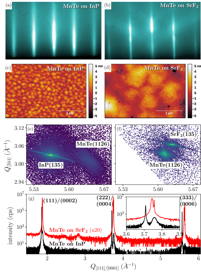
FIG. 2. Reflection high-energy electron diffraction (RHEED) patterns of 50-nm and 2500-nm thick epitaxial MnTe films on InP(111)A (a) and SrF 2 (111) (b), respectively, recorded along the [\bar{1}\bar{1}0] zone axis. Atomic force microscope images for MnTe films on InP(111)A and SrF 2 (111) are shown in (c) and (d). X-ray diffraction reciprocal space maps around the (135) substrate Bragg reflection of the samples are shown in (e) and (f). Due to the epitaxial relationship, the (11 \bar{2} 6) Bragg reflection of MnTe is seen close to the substrate peaks. (e) shows the symmetric radial scan for MnTe on InP (black) and MnTe on SrF 2 (red). For clarity, the trace of MnTe on SrF 2 was scaled by a factor of 20. The inset shows a zoom around the (222) substrate Bragg peaks and the broader (0004) Bragg peaks of the MnTe epilayer. Data in (c)–(e) are recorded at room temperature where due to different strain states the Bragg peak position of the films is slightly different for the two used substrate materials.
