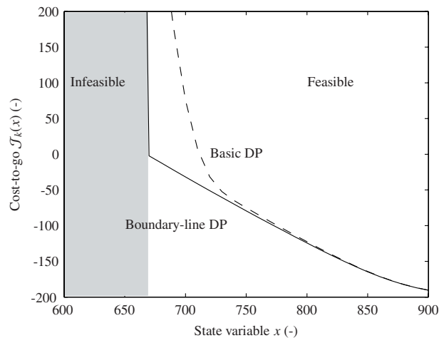
Figure 2 Section of the cost-to-go function \mathcal{J}_k(x) at time index k such that t = 180 h for the fishing problem. State-space discretization is \Delta x = 10 , penalty for infeasible states is set to \mathcal{J}_\infty = 1200 .
