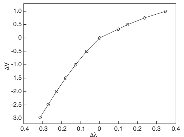
Figure 2 UEGO sensor calibration curve.
