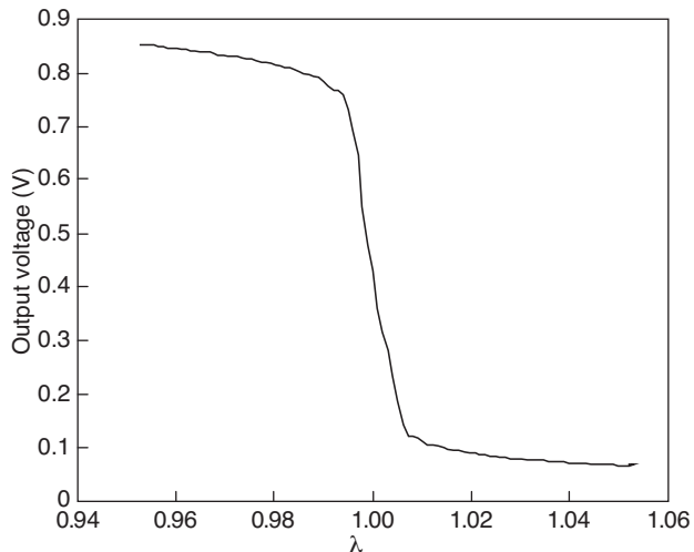
Figure 1 HEGO sensor response as a function of AFR, \lambda .
