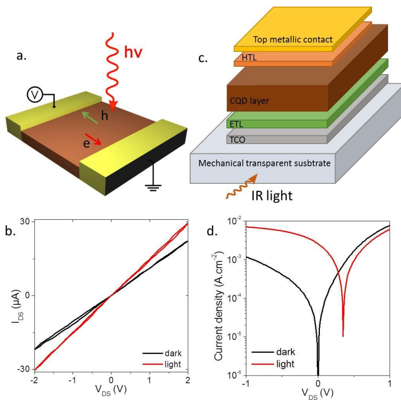
Figure 1 a. Scheme of a photoconductive device in planar geometry. b. I-V curve of a photoconductive device under dark condition and under illumination. c. Scheme of a photodiode in vertical geometry. TCO, ETL and HTL stands respectively for transparent conductive oxide, hole transport layer and electron transport layer. d. I-V curve of a photodiode under dark condition and under illumination.
