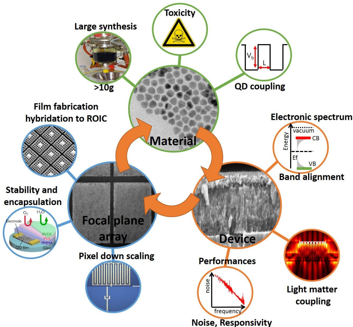
Figure 2 : Illustration of the main challenges that need to be addressed to bring the field of IR nanocrystals to a mature level for thermal imaging.
