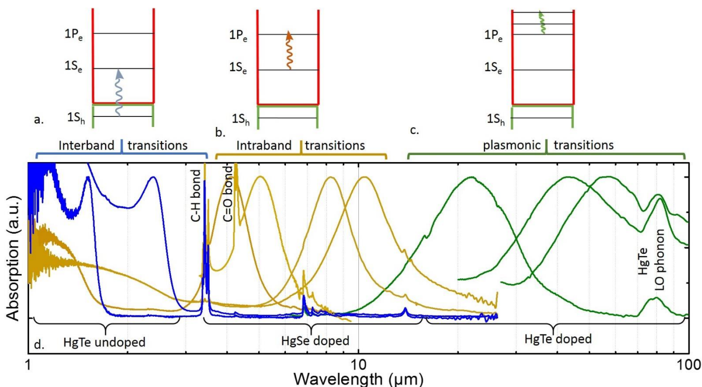
Figure 3 a, b and c are respectively the scheme for interband, intraband and plasmonic transitions in nanocrystals. d. Absorption spectra for mercury chalcogenide (HgSe and HgTe) nanocrystals of various sizes
