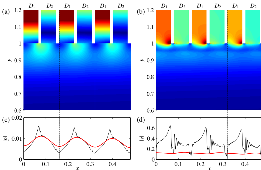
FIGURE 9. (Colour online) Iso-colour plots of the amplitudes of (a) pressure and (b) v -velocity for 3 periodic cells when the Bloch mode ( k_B = 10.056 - 0.3252i ) propagates in the lined duct. The vertical dashed lines denote the boundaries of the periodic cells. Each cell consists of two cavities with different depths: D_1 = D - d and D_2 = D + d , where d = 0.04 ( d^* = 0.6 mm). (c) and (d) show the amplitudes of pressure and v -velocity as a function of x at 2 different y -positions: black thin lines for y = 1 - \Delta h/2 , and red thick lines for y = 0.9525 where the mean flow velocity equals to the wave velocity of k_B . The calculations are made at frequency \omega = 0.4310 . Note that the fields are only plotted for part of the duct and the liner cavities.
