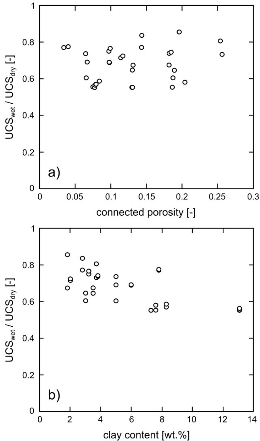
Figure 6. (a) The ratio of wet to dry uniaxial compressive strength for the twelve sandstones sampled from exploration well EPS-1 at Soultz-sous-Forêts and the three quarry rocks as a function of connected porosity. (b) The ratio of wet to dry uniaxial compressive strength for the twelve sandstones sampled from exploration well EPS-1 at Soultz-sous-Forêts and the three quarry rocks as a function of clay content (clay content is the wt.% of muscovite/illite-smectite; Table 1).
