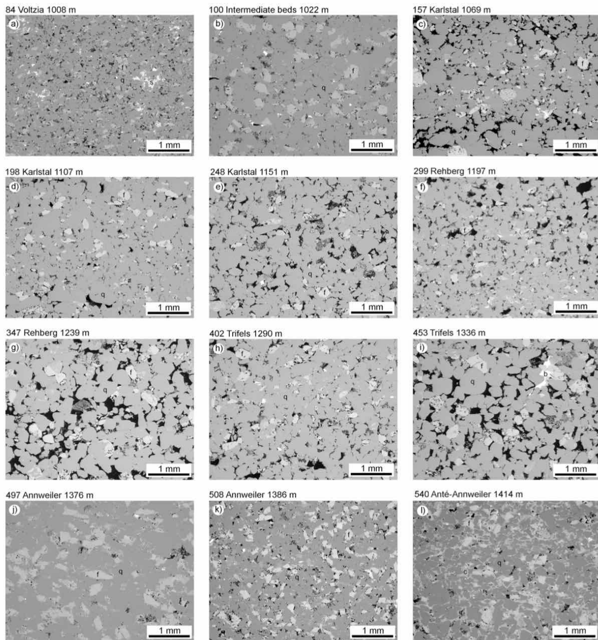
Figure 3. Backscattered scanning electron microscope (BSE) images for each of the twelve sandstones sampled from exploration well EPS-1 at Soultz-sous-Forêts. The box number, lithological unit, and depth are given above each image. q – quartz; f – feldspar; s – siderite; b – barite; c – clay.
