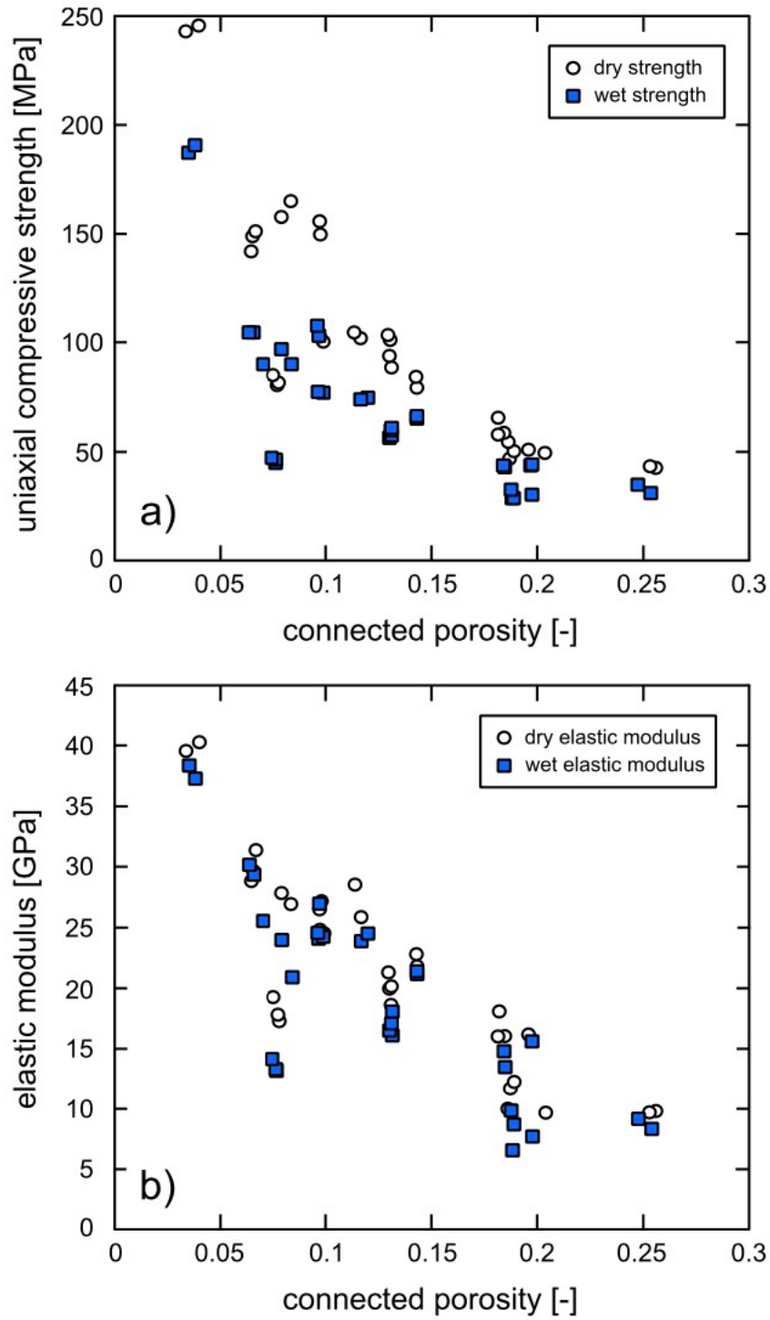
Figure 5. (a) Dry (white circles) and wet (blue squares) uniaxial compressive strength for the twelve sandstones sampled from exploration well EPS-1 at Soultz-sous-Forêts and the three quarry rocks as a function of connected porosity. (b) Dry (white circles) and wet (blue squares) elastic modulus for the twelve sandstones sampled from exploration well EPS-1 at Soultz-sous-Forêts and the three quarry rocks as a function of connected porosity.
