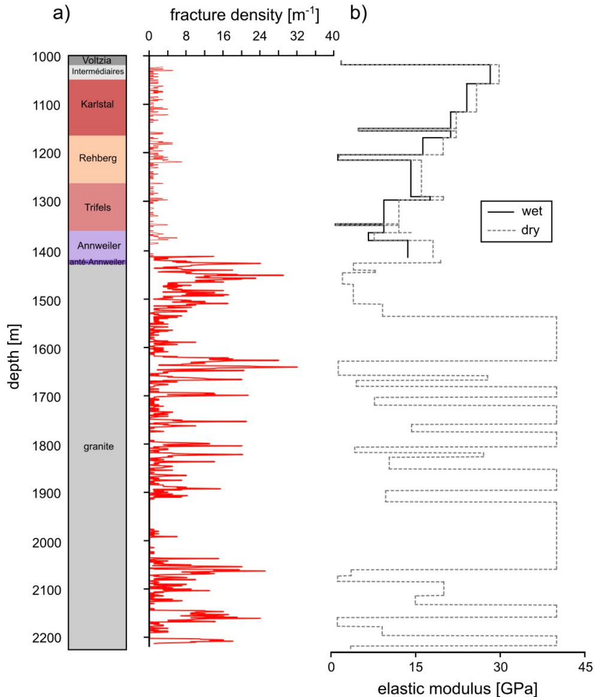
Figure 15. (a) Stratigraphic column of exploration well EPS-1 at Soultz-sous-Forêts (from 1012 to 2200 m) next to the fracture density data for the core. (b) Wet (black line) and dry (grey dashed line) rock mass elastic modulus. Note that dry and wet values are given for the Bundsandstein (interval 1012-1416 m) only.
