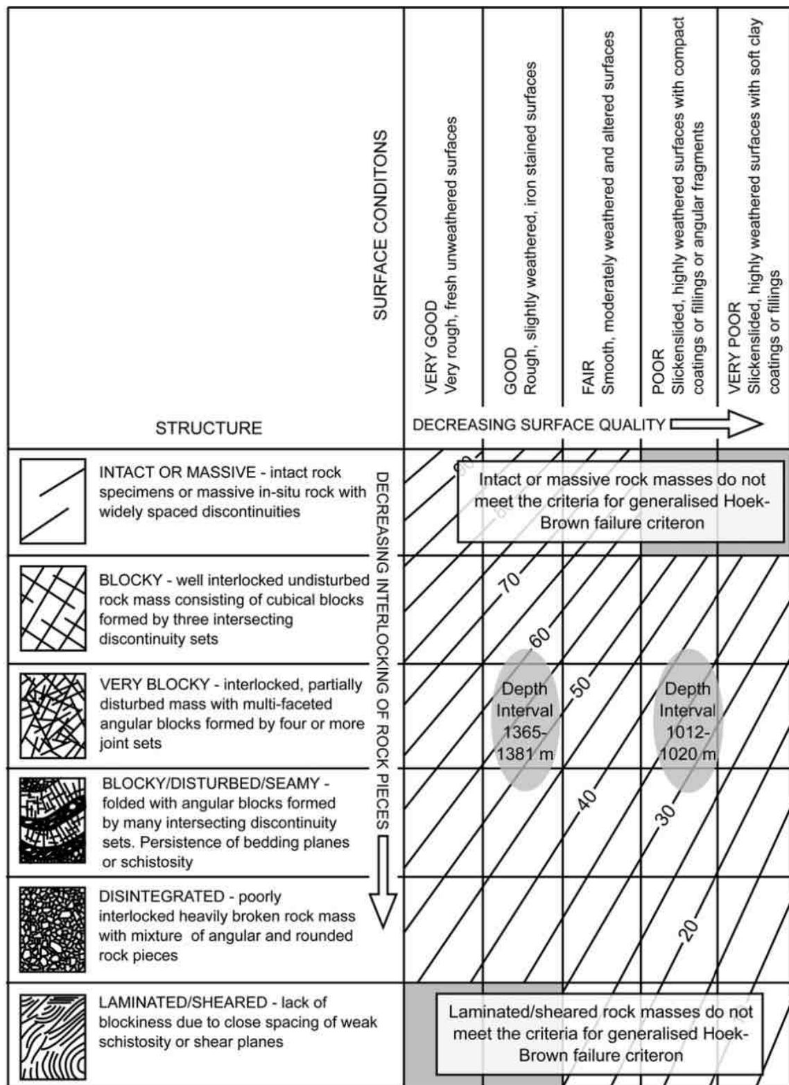
Figure 10. Geological Strength Index (GSI) lookup chart (modified from Marinos et al., 2005) showing the assessed GSI values for two rock mass intervals (see text for details). See Table 5 for rock mass descriptions based on core logging. Note that the highest and lowest category should not be used for the generalised Hoek-Brown failure criterion (as indicated on the figure).
