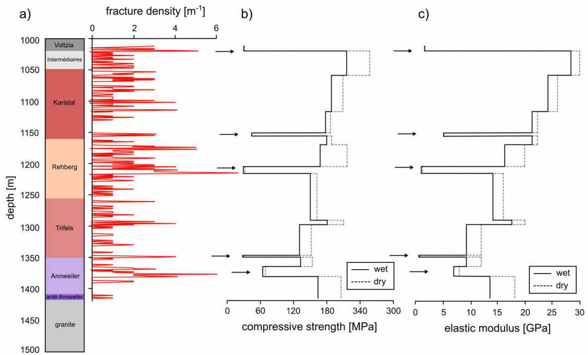
Figure 11. (a) Stratigraphic column showing the units within the Buntsandstein from exploration well EPS-1 at Soultz-sous-Forêts next to the fracture density data for the core. (b) Wet (black line) and dry (grey dashed line) rock mass compressive strength for the Buntsandstein over the depth interval 1012-1416 m. (c) Wet (black line) and dry (grey dashed line) rock mass elastic modulus for the Buntsandstein over the depth interval 1012-1416 m. The black arrows indicate the five fractured zones.
