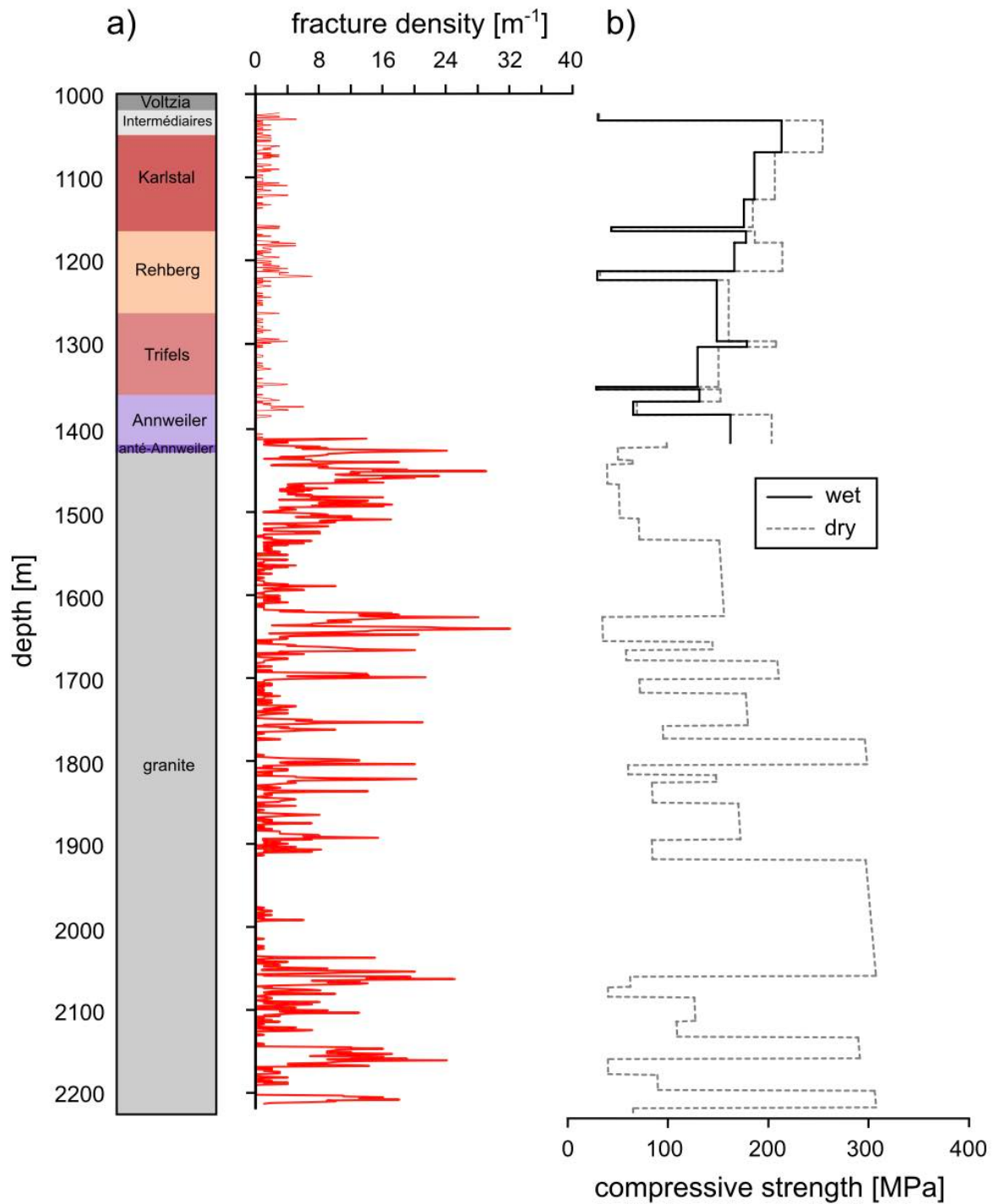
Figure 14. (a) Stratigraphic column of exploration well EPS-1 at Soultz-sous-Forêts (from 1012 to 2200 m) next to the fracture density data for the core. (b) Wet (black line) and dry (grey dashed line) rock mass compressive strength. Note that dry and wet values are given for the Bundsandstein (interval 1012-1416 m) only.
