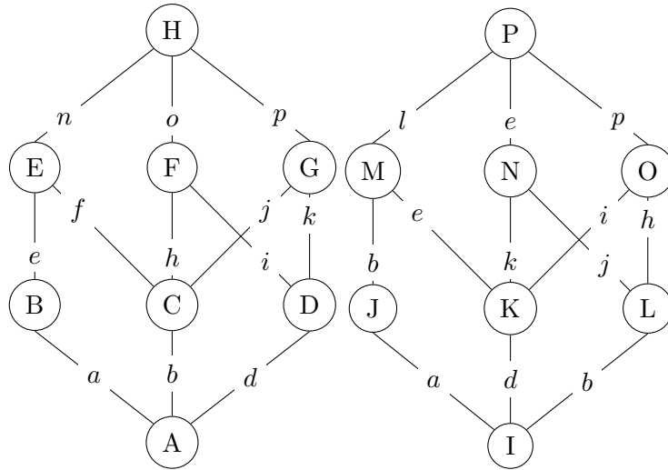
FIGURE 7. Second counter-example
