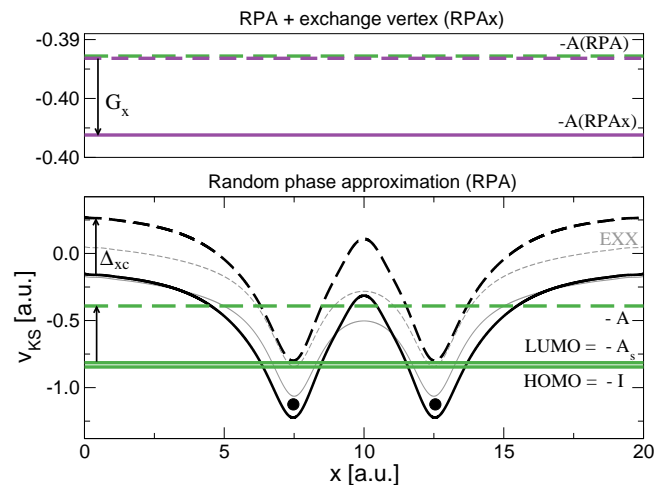
FIG. 2. Lower panel: KS potential of a soft-Coulomb stretched \text{H}_2 molecule in the RPA approximation (black full and dashed curves). Horizontal lines indicates the KS HOMO and LUMO energy levels (green full) and the corrected affinity (green dashed). EXX approximation in the background (grey curves). Upper panel: RPAX corrected affinity (purple dashed and full lines are without and with discontinuity, respectively).
