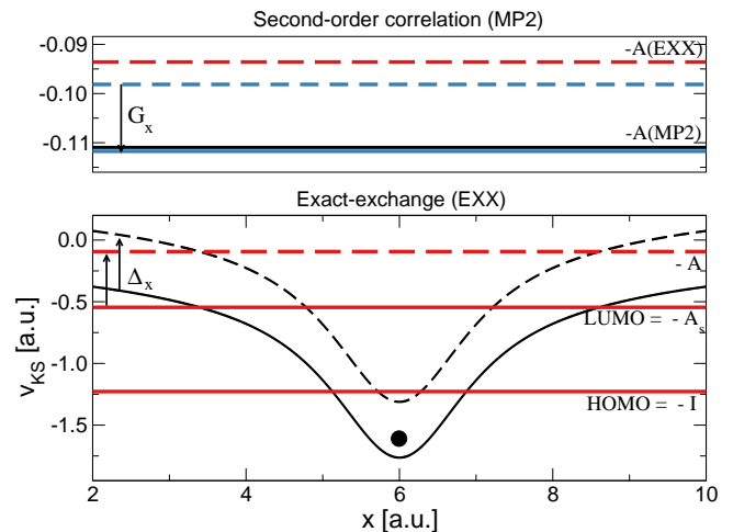
FIG. 1. Lower panel: KS potential of a soft-Coulomb two-electron atom in the EXX approximation (black full and dashed curves). Horizontal lines indicates the KS HOMO and LUMO energy levels (red full) and the corrected affinity (red dashed). Upper panel: MP2 corrected affinity (blue dashed and full lines are without and with discontinuity, respectively). Black full line is the nonlocal MP2 result.
