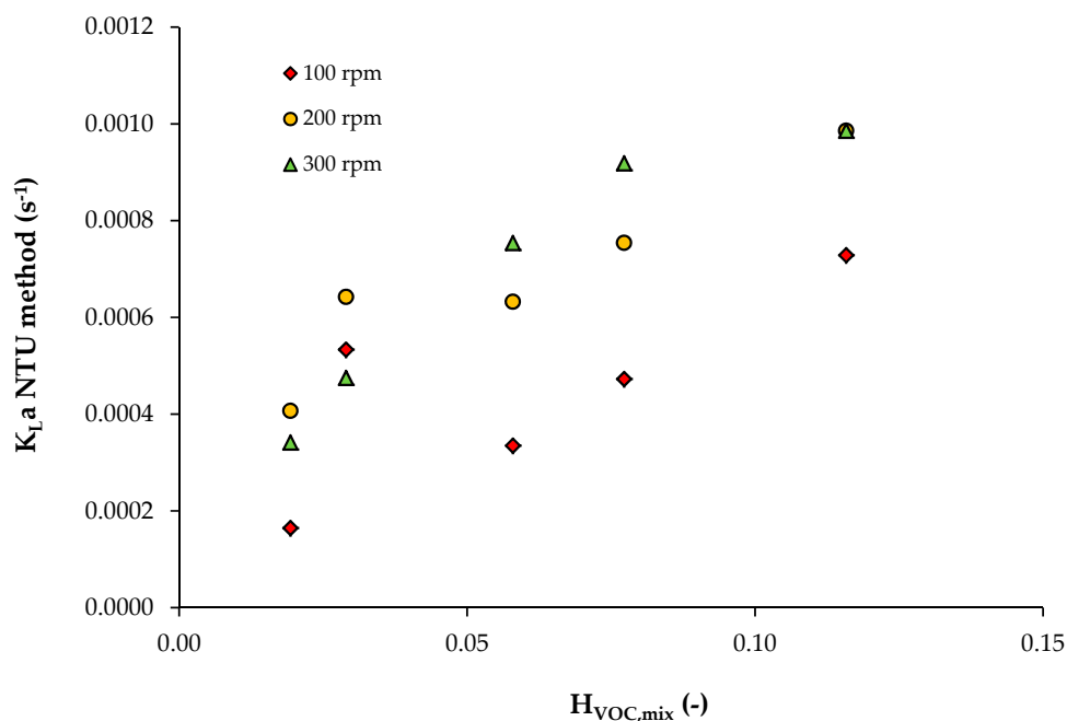
Figure 6. K_{\text{L}}a vs. Henry coefficient from data reported in Bordel et al. [28].
