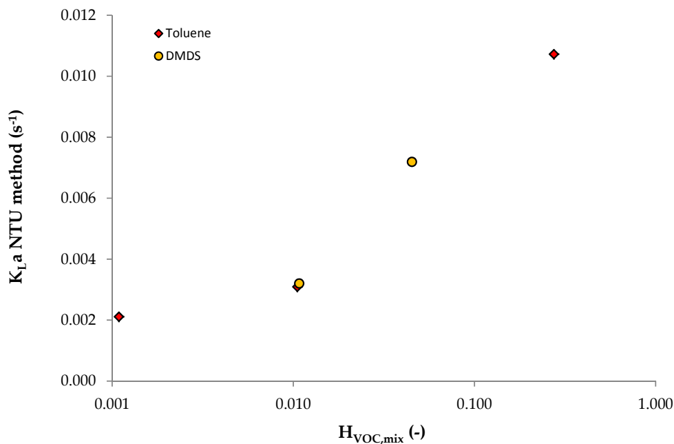
Figure 4. K_{L,a} vs. Henry coefficient from data reported in Dumont et al. [11] (gas flow-rate = 5.19 \times 10^{-3} \text{ m}^3/\text{s} ; gas EBRT = 2.2 s; liquid flow-rate = 10^{-4} \text{ m}^3/\text{s} ; V = 1.13 \times 10^{-2} \text{ m}^3 ; T = 25 \text{ }^\circ\text{C} ).
