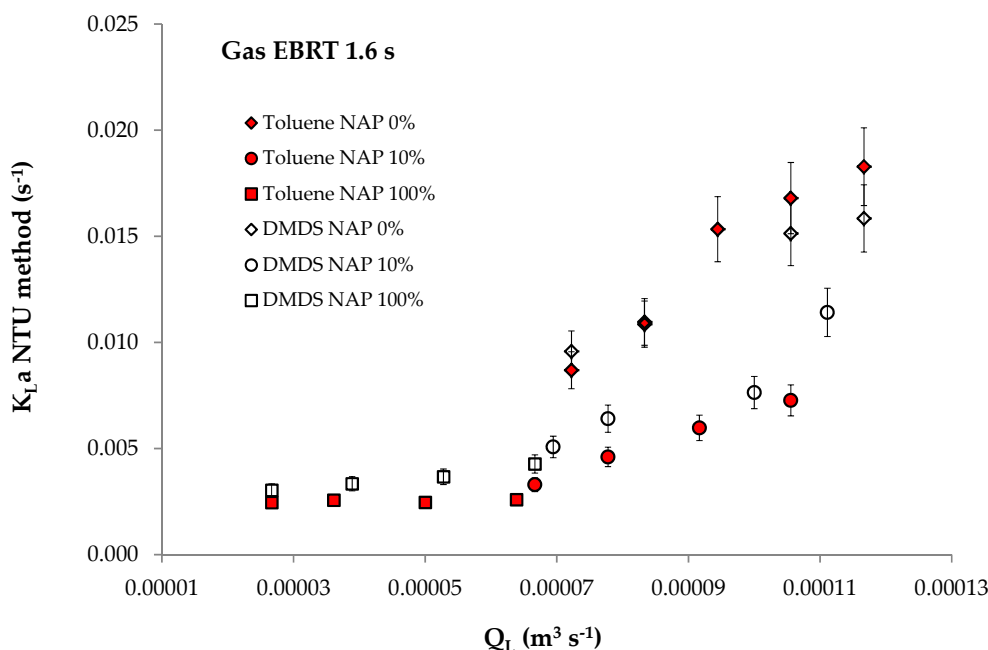
Figure 3. K_L a vs. liquid flow-rate from data reported in Dumont et al. [11] (gas flow-rate = 7.3 \times 10^{-3} m^3/s ; V = 1.13 \times 10^{-2} m^3 ; T = 25^\circ C ).
