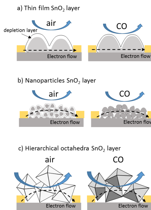
Figure 6. Schematic cartoon of the intergrains electrical modulation under air and CO exposure in thin film (a), nanoparticles (b) and octahedra (c).
