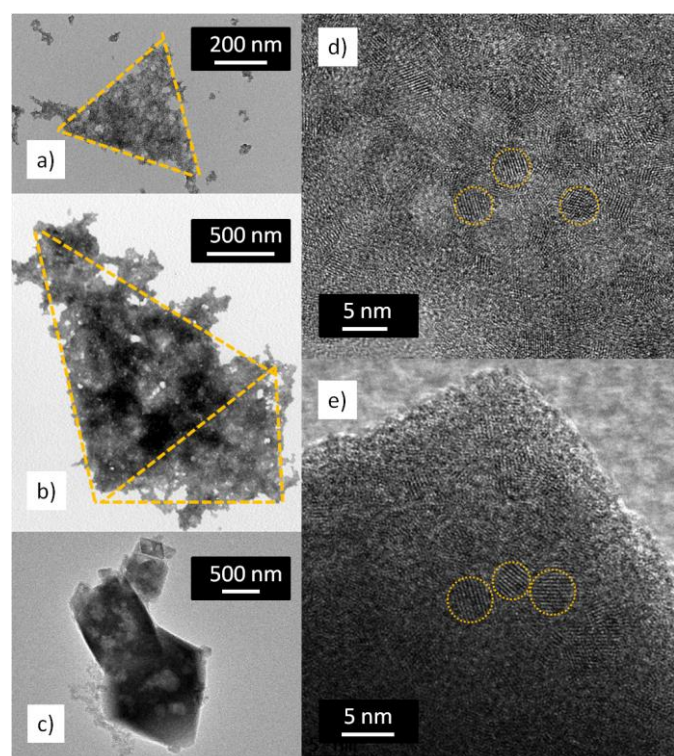
Figure 3. TEM image of \text{Sn}_3\text{O}_2(\text{OH})_2 triangular sheets after 5 min (a) and 7h (b) of reaction (c), HRTEM image of the \text{Sn}_3\text{O}_2(\text{OH})_2 octahedra obtained after 16h of reaction (c), HRTEM image of \text{Sn}_3\text{O}_2(\text{OH})_2 nanocrystalline triangular sheets (d), HRTEM image of \text{Sn}_3\text{O}_2(\text{OH})_2 nanocrystalline octahedra facet (e).
