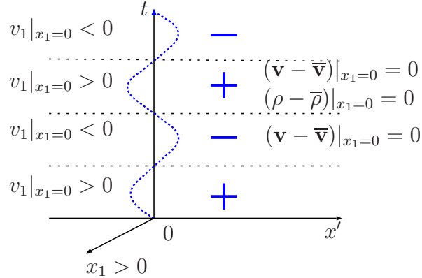
Figure 2: Periodic subsonic inflow-outflow boundary conditions for the Navier-Stokes system.
